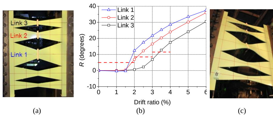
Figure 10 Behavior of Pair 10 with combination: (a) front view before loading; (b) angle of rotation ( R ) versus drift ratio relationship; (c) upward view after 2 cycles of 3.5%.
