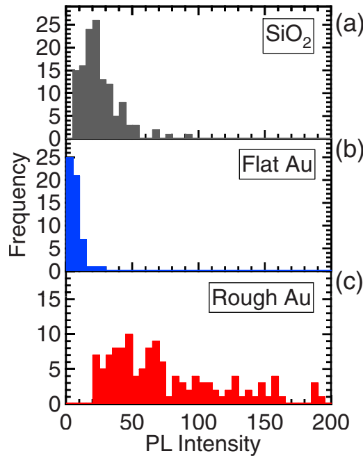
FIG. 2. (Color online) [(a)–(c)] Histograms of the PL intensity of about 100 single carbon nanotubes on fused silica, flat Au, and rough Au surfaces, respectively. The rough Au substrate has a PMMA layer of 15 nm.
