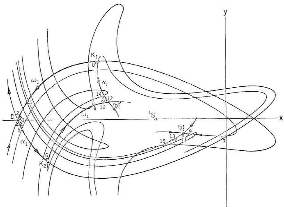
(b) A heteroclinic cycle: K_1\omega_1(D)D\alpha_1(D)K\omega_1({}^2D_1^2){}^2D_1^2\alpha_1({}^2D_1^2)K_1 .
