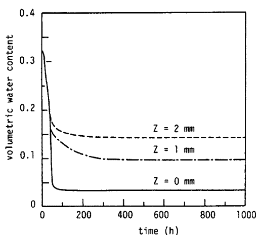
Fig. 3. Changes of the water content near the ground surface with time in the case of Exp. A(1).
