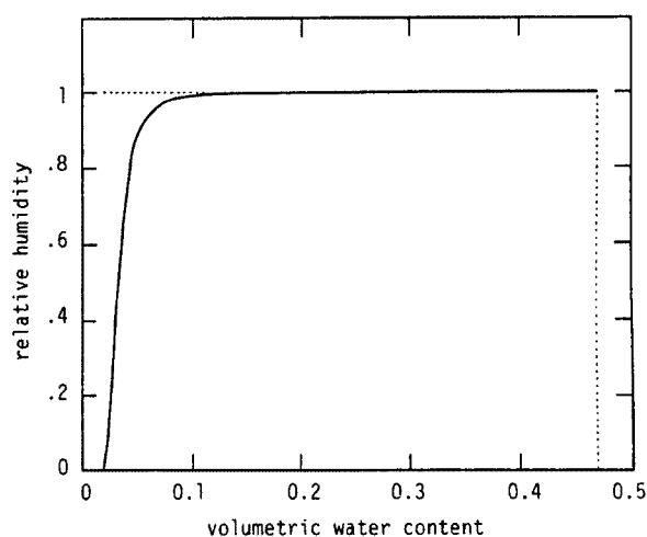
Fig. 4. Relation between the relative humidity and the water content for the soil S-1.
