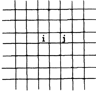
Figure 1: Square lattice and Nearest Neighbor.
