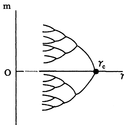
Figure 4: Order parameter bifurcates and multiple equilibria.
