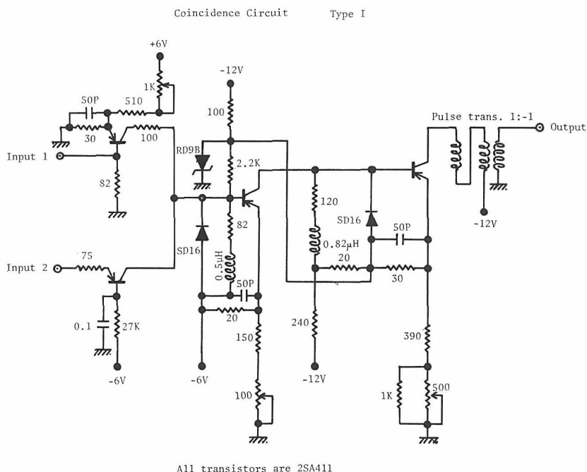
Fig. 17. Block diagram of the coincidence circuit of type I.
