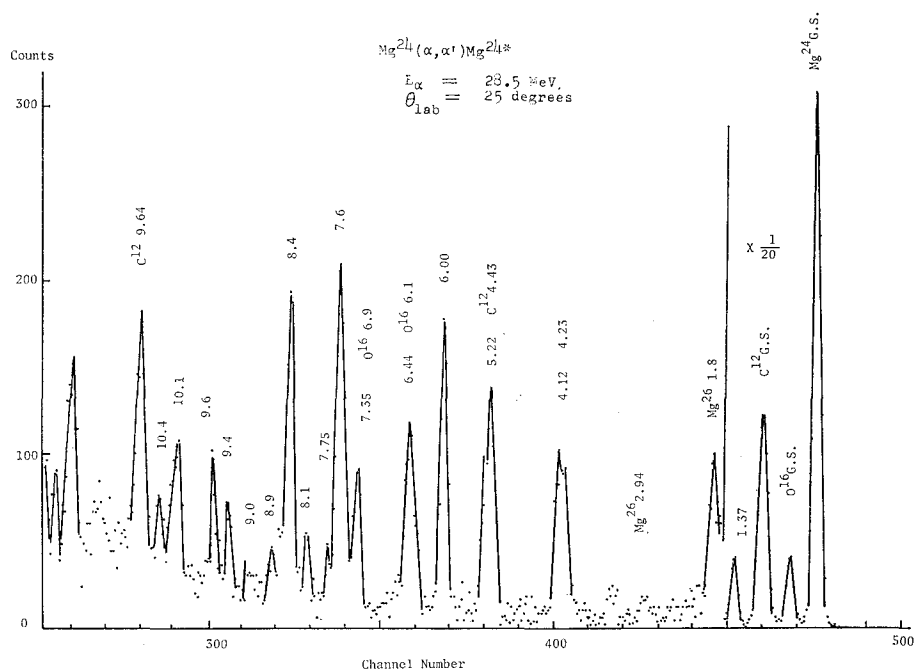
Fig. 2. A typical pulse height spectrum of alpha particles from the reaction ^{24}\text{Mg}(\alpha, \alpha')^{24}\text{Mg}^* using the pre-amplifier of type I.
