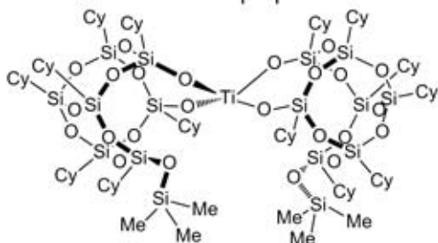
1b (Cy = c\text{-C}_5\text{H}_9 )
