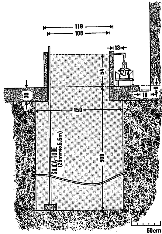
Fig. 2. Structure of the observation pit.
