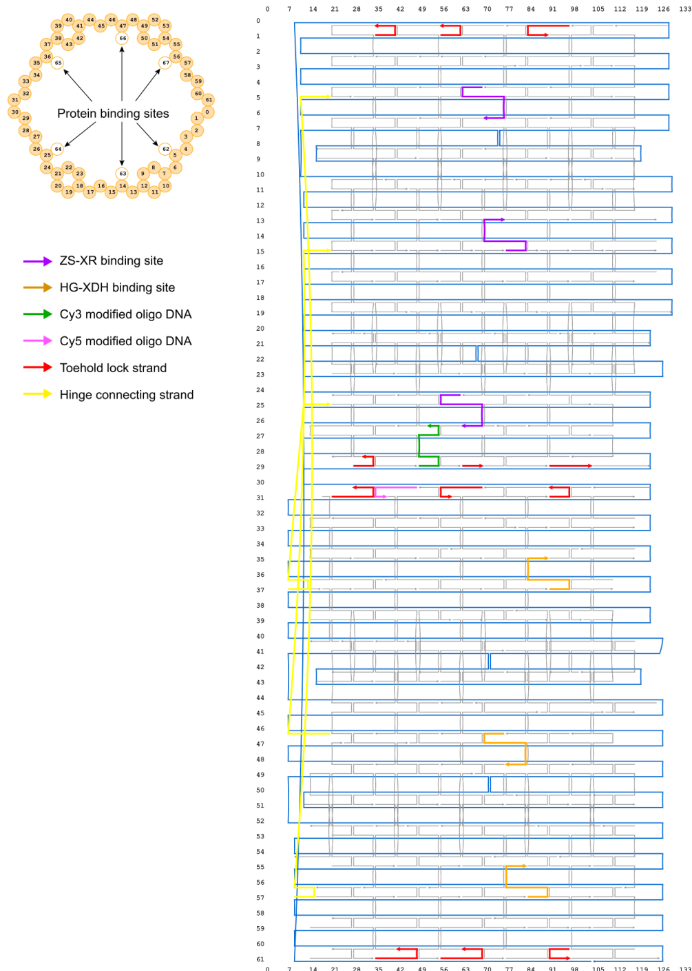
Figure 5.28. Front view and blueprint modified from caDNA 47 software interface of DNA scaffold ( http://cadnano.org/ ) with the extension positions of toehold locks. The staple strands in purple and orange indicated enzyme ZS-XR and HG-XDH attachment sites, respectively. The staple strands in green and pink were Cy3-modified oligo and Cy5-modified oligo, respectively. The staple strands in red were the positions for the extension positions of toehold lock sequences. The staple strands in yellow were connecting hinges when used for the folding of DNA scaffold in open state in 180°.
