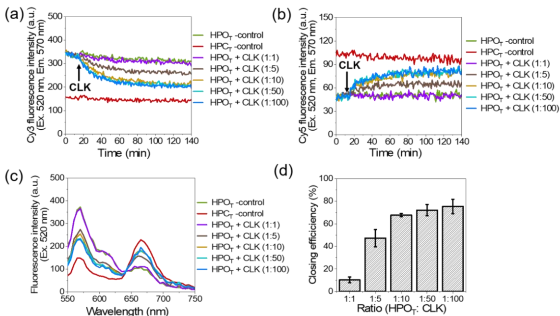
Figure 5.9. The effect of molar ratio ( \text{HPO}_T : CLK) on the closing efficiency. (a) Time course changes of the Cy3 fluorescence intensity ( \lambda_{\text{ex}} = 520 \text{ nm} , \lambda_{\text{em}} = 570 \text{ nm} ) of closing procedure. (b) Time course of Cy5 fluorescence intensity ( \lambda_{\text{ex}} = 520 \text{ nm} , \lambda_{\text{em}} = 670 \text{ nm} ) of closing procedure. (c) Fluorescence emission spectra ( \lambda_{\text{ex}} = 520 \text{ nm} ) after 2-h hybridization at 25 °C. (d) Closing efficiency calculated from the Cy5 fluorescence intensity in the fluorescence emission spectra after 2-h hybridization at 25 °C. 5 nM \text{HPO}_T was hybridized with 5 nM to 500 nM CLK in the buffer (pH 7.0) containing 40 mM Tris-HCl, 20 mM acetic acid, 12.5 mM \text{MgCl}_2 and 0.002% Tween20 at 25 °C. Data in (d) were the averages of three independent repetitions, error bars indicated the S.D. of the repetitions.
