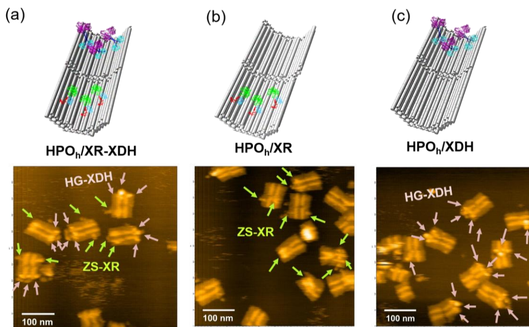
Figure 5.20. Assembly of enzymes on the statically open state of DNA scaffold ( \text{HPO}_h ). (a) An illustration and typical AFM image of \text{HPO}_h/\text{XR-XDH} , scale bar: 100 nm. (b) An illustration
