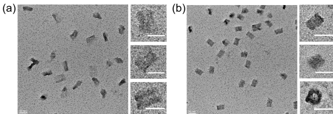
Figure 5.5. TEM images of the DNA scaffold. (a) TEM images of DNA scaffold in the open state (HPO T ), scale bar: 50 nm. The expanded images of typical open state were shown in right side, scale bar: 50 nm. (b) TEM images of DNA scaffold in the closed state (HPC T ), scale bar: 50 nm. The expanded images of typical closed state were shown in the right side, scale bar: 50 nm. The well-formed yield of closed state was estimated to be 92% (187/203) from TEM images.
