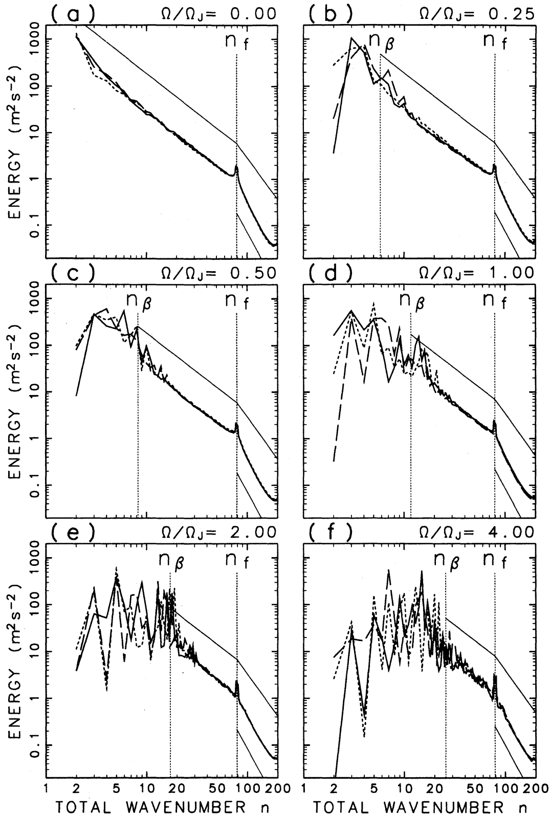
Fig.3: Energy spectrum \overline{E}(n) averaged from 800 to 1000 J.days for six values of \Omega/\Omega_J . The forcing wavenumber is indicated by n_f and the wavenumber n_\beta is also indicated, at which scale the “ \beta -term” is comparable to the nonlinear Jacobian term. Three spectra are plotted for each figure. The spectrum obtained with the same random numbers is plotted with the same line type. A line of \overline{E}(n) \propto n^{-5/3} is added in the range of n_\beta \leq n \leq n_f , and lines of n^{-3} (above) and n^{-4} (below) are also added in the range of n_f \leq n \leq N .
