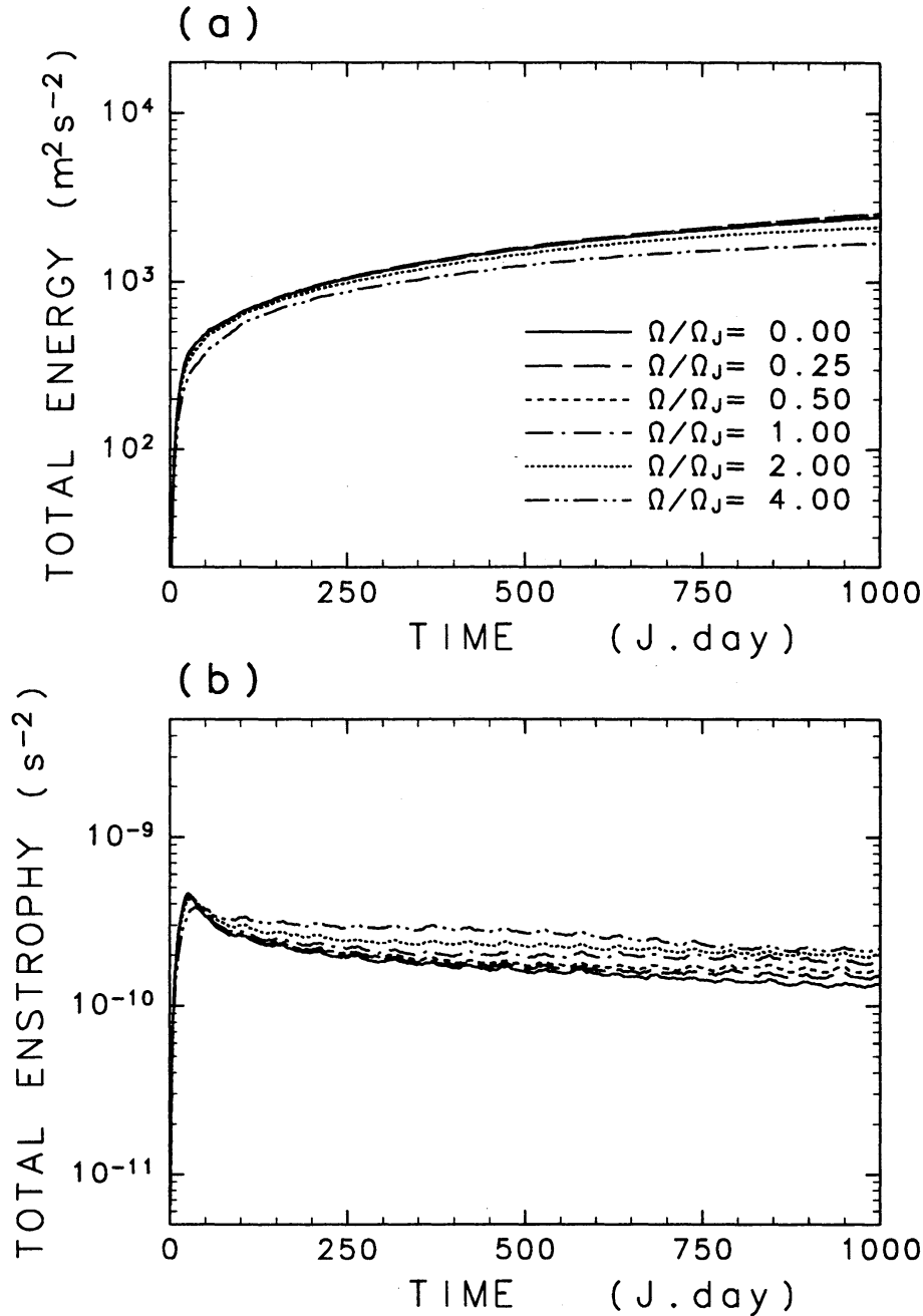
Fig.2: Temporal variation of the total kinetic energy \mathcal{E}(t) (a), and the total enstrophy \mathcal{Q}(t) (b) for six values of \Omega/\Omega_J . Ensemble averages of three runs.
