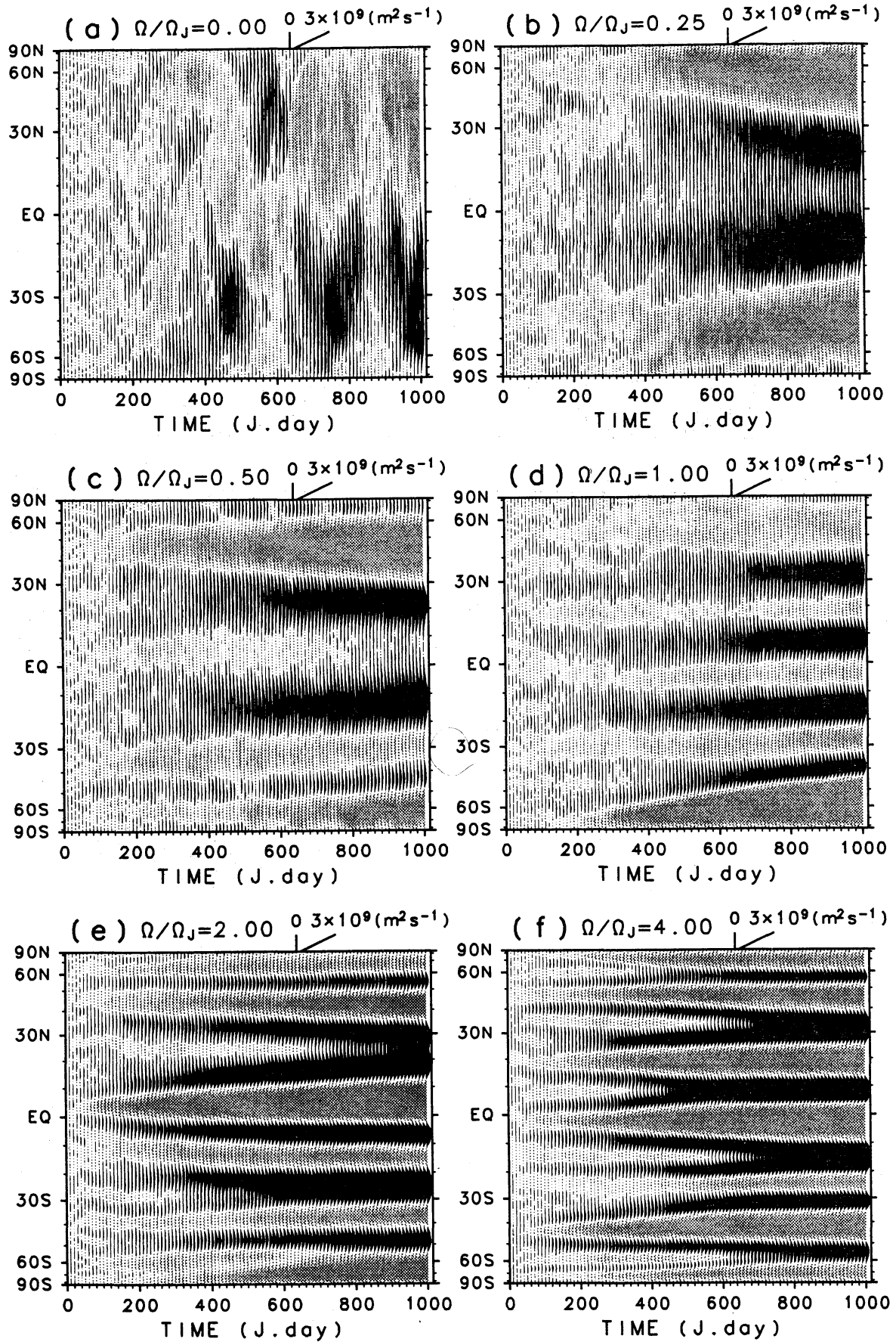
Fig.6: Temporal variation of the zonal mean angular momentum for the same runs as in Fig.5. Time interval is 10 J.days, and the unit of an interval is 3 \times 10^9 \text{ m}^2 \text{ s}^{-1} . Westerly zones are in black while easterly zones in gray.
