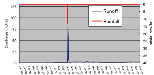
Fig.16 Daily discharge simulation hydrograph and rainfall hyetograph.
