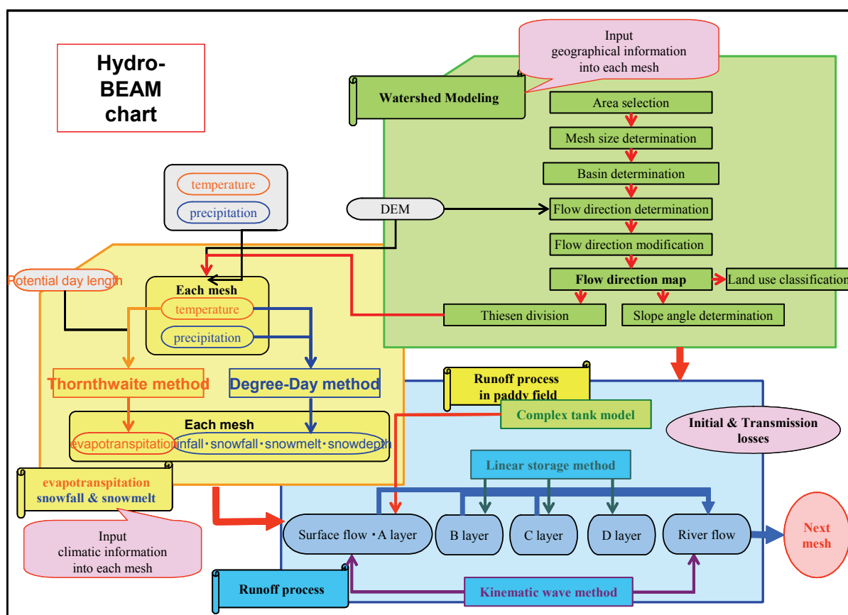
Fig. 9 Hydro-BEAM flow chart
