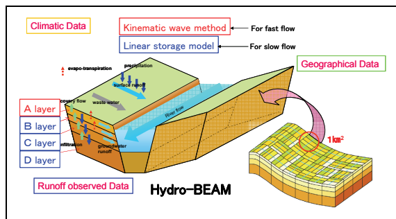
Fig. 6 Conceptual model of Hydro-BEAM
