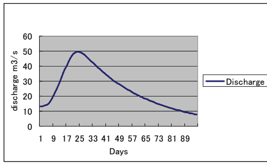
Fig. 17 Hydrograph of hourly discharge simulation
