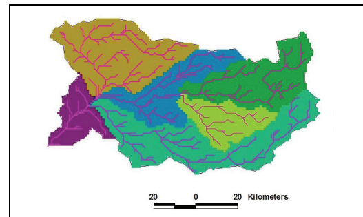
Fig. 7 Watershed delineation and stream network determination of Wadi Assiut
