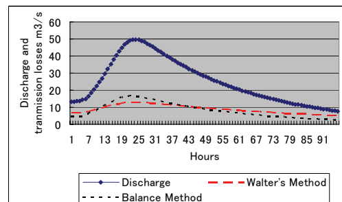
Fig.21 Comparing of discharge and transmission losses (Walter's Equation and Balance method)
