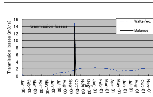
Fig.20 Transmission losses simulation (Walter's Equation and Balance method)
