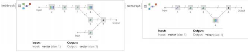
Figure 2: net11 , net12
