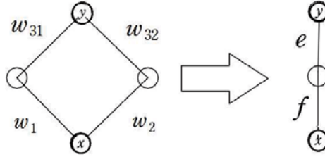
Figure 1: H = 2 \Rightarrow H_0 = 1
