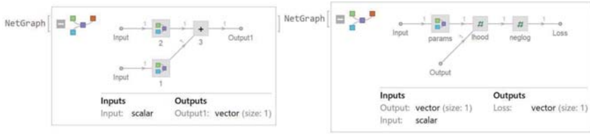
Figure 3: parameterNet, trainingNet
