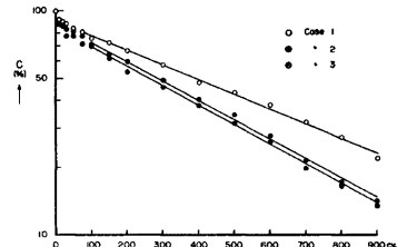
Fig. 13. Time change of average dye concentration in Seto Inland Sea.
