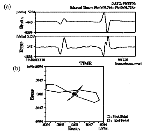
Fig. 4: (a) Waveforms of the parallel (upper panel) and perpendicular (lower panel) electric field with respect to the ambient magnetic field observed in the upstream region of the bow shock during the period from 19:40:00.716 UT to 19:40:00.728 UT on October 06, 1997 by the WFC receiver, and (b) corresponding hodograph of the observed electric field.
