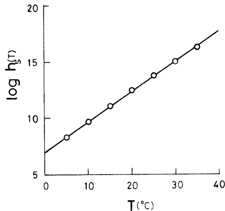
Fig. 30 飽和絶対湿度と温度の関係 \log h_s(T) = \log 4.983 + 0.0269T , r = 0.9997
