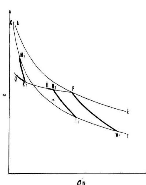
Fig.4.15. e-\sigma'_m relations in drained triaxial compression test
