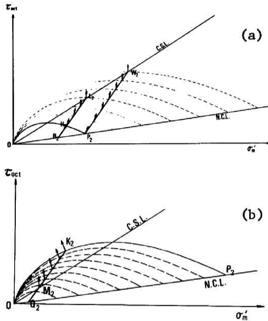
Fig.5.17. Stress paths and plastic strain increments ( \sigma_a : increase, \sigma_r : constant) (a) wetter than critical (b) drier than critical
