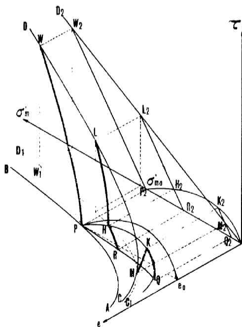
Fig.4.14. State paths in drained triaxial compression test
