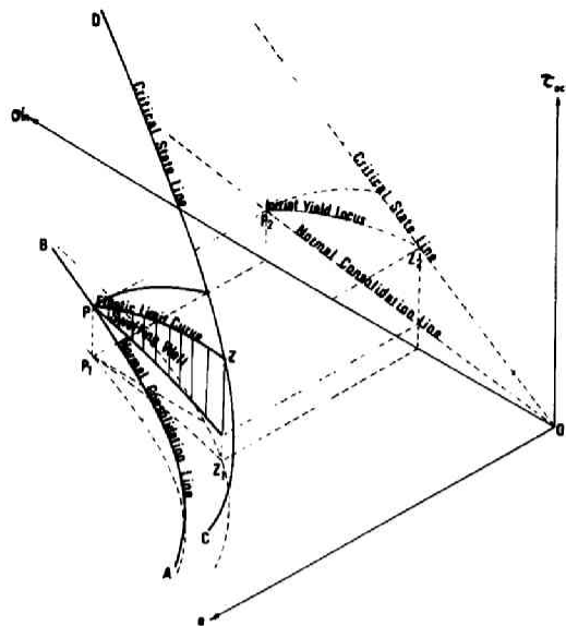
Fig.5.2. Swelling wall of anisotropically consolidated clay (wetter side)
