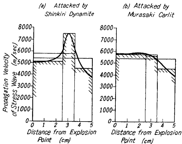
Fig. 16. Change of velocity in marble against the distance from the explosion point.
