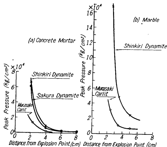
Fig. 19. Changes of peak pressure with the distance from explosion point.
