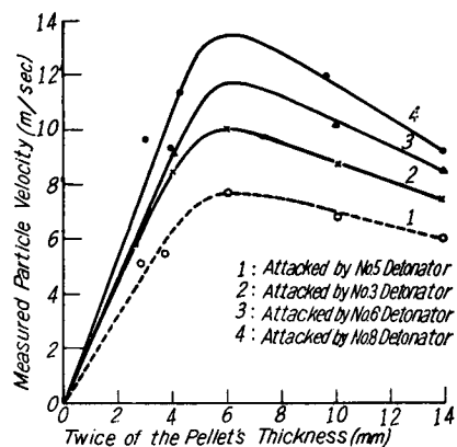
Fig. 5. Measured particle velocities for sandstone.
