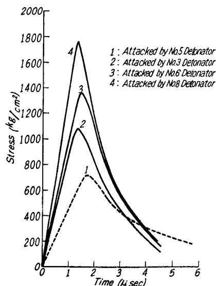
Fig. 7. Stress wave shapes for sandstone.
