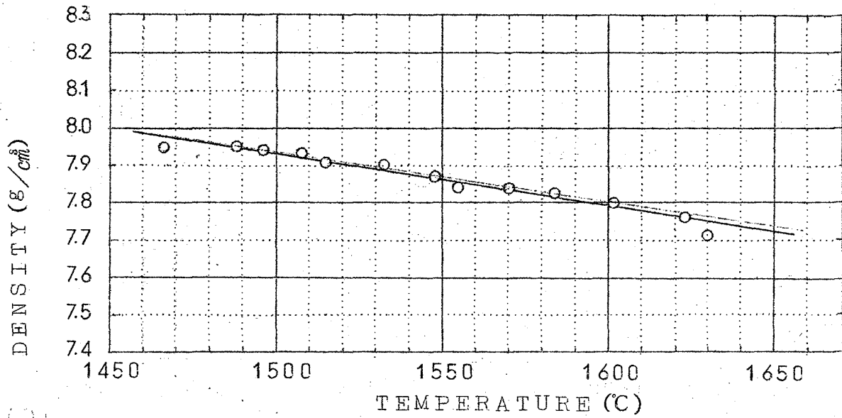
Fig. 7 Density of liquid nickel
