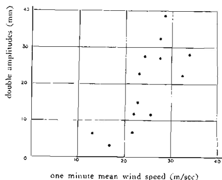
Fig. 4 The relation between amplitudes and wind speed averaged over one minute.
