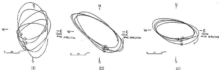
Fig. 3 Movement at the top of the tower.
