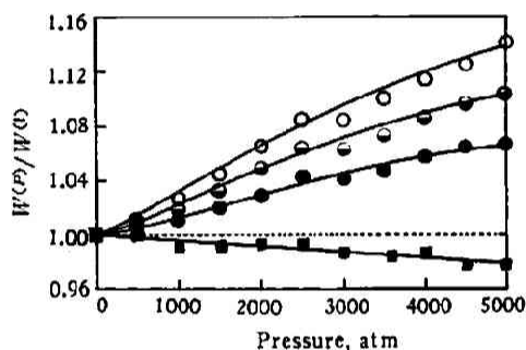
Fig. 3. Variation of the Walden products with pressure at 25°C ○: W^{(P)}(\text{Cl}^-) , ○: W^{(P)}(\text{KCl}) ●: W^{(P)}(\text{K}^+) , ...: W^{(P)}(\text{Bu}_4\text{N}^+) ■: W^{(P)}(\text{Me}_4\text{N}^+)
