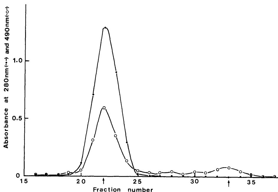
Fig. 2. Gel filtration of the aldobiouronic acid-methylated BSA conjugate on Sephadex G-25 column. The arrows represent the void volume and the elution volume of the aldobiouronic acid, respectively.
