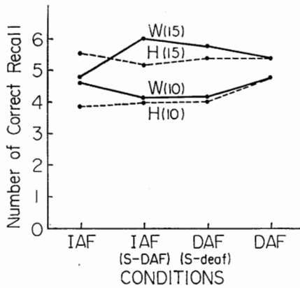
Fig.2 Number of Immediate Free Correct Recall
