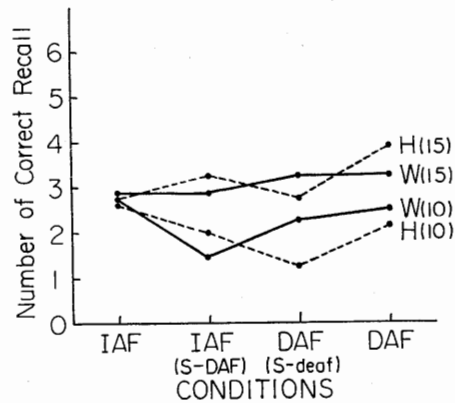
Fig.3 Number of Delayed Free Correct Recall
