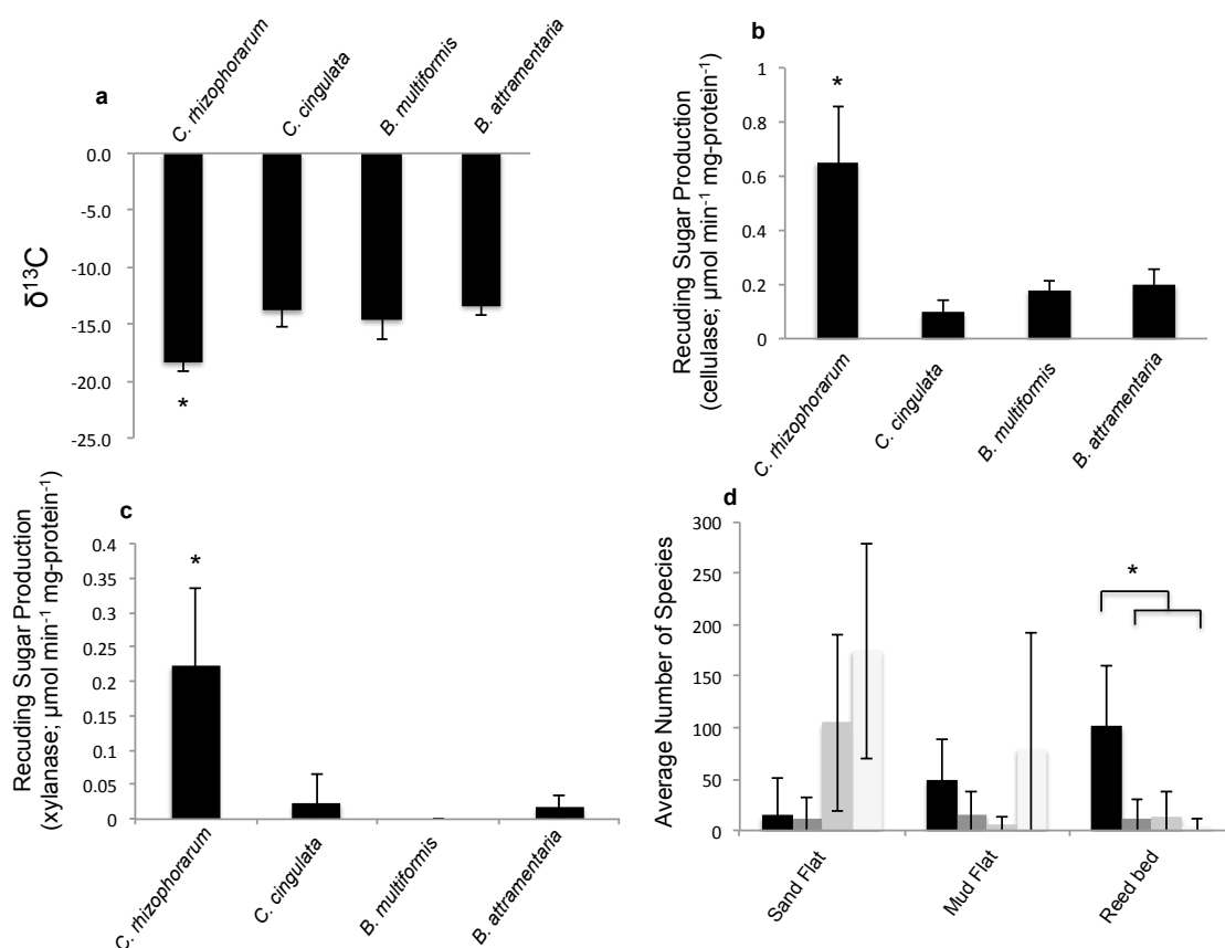
Fig. 2-5 Comparison of \delta^{13}\text{C} value, cellulase activity, xylanase activity, and spatial distribution among 4 species of gastropods. Bars represent SEM. (a), \delta^{13}\text{C} value; (b), cellulase activity; (c), xylanase activity; (d), spatial distribution. Error bars represent SD; asterisks indicate significant differences. Bars in (d): black, Cerithidea rhizophorarum ; dark gray, Cerithidea cingulata ; gray, Batillaria multiformis ; white, B. attramentaria .
