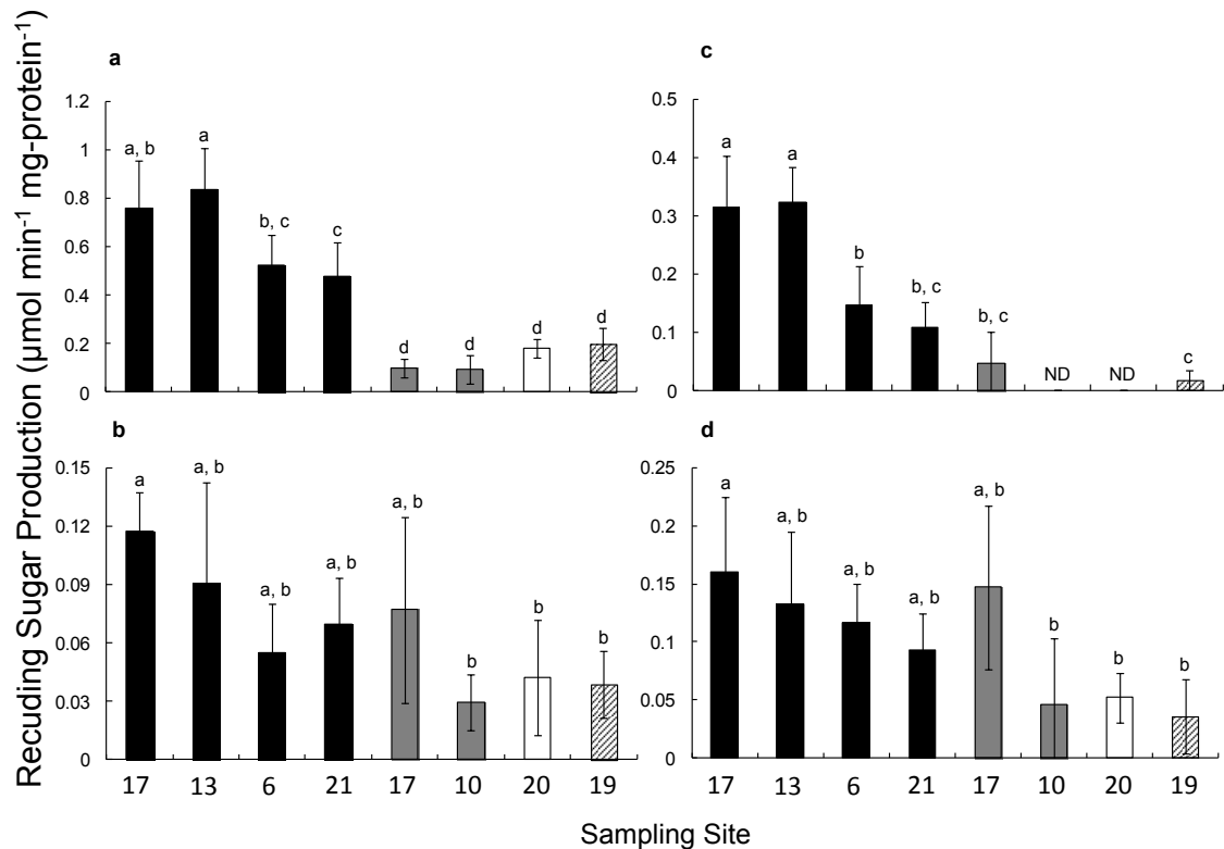
Fig. 2-2 Cellulase and hemicellulase activities in the digestive glands of Cerithidea rhizophorarum after incubation of tissue extracts with appropriate substrates. a, cellulase activity; b, mannanase activity; c, xylanase activity; d, laminarinase activity. Bars represent SEM. ND, not detectable. Black, Cerithidea rhizophorarum ; gray, Cerithidea cingulata ; white, Batillaria multiformis ; striped pattern, B. attramentaria . Values followed by the same letters do not differ significantly (Tukey's HSD, p < 0.05 ).
