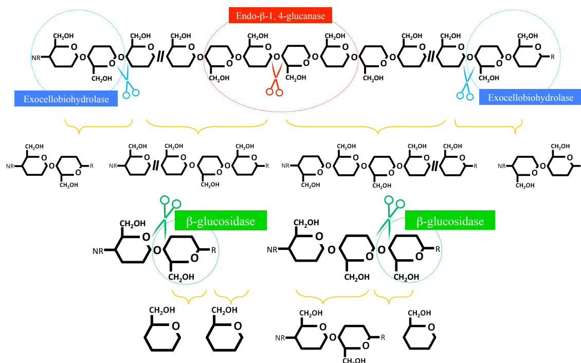
Fig. 0-2 Three types of cellulose hydrolysis enzymes that are collectively called cellulases, namely exocellobiohydrolase, endo- \beta -1, 4-glucanase, and \beta -glucosidase. Exocellobiohydrolases (exocellulase) cleave cellulose to release cellobiose from reducing (R) or nonreducing (NR) termini (dotted circle). Endo- \beta -1, 4-glucanases cleave the cellulose randomly at internal \beta -1, 4 linkages (broken circle). \beta -Glucosidases hydrolyze cellobiose or cello-oligomersto to release glucose from the reducing temini (double circle). Scissors represent the cutting site of each enzyme.
