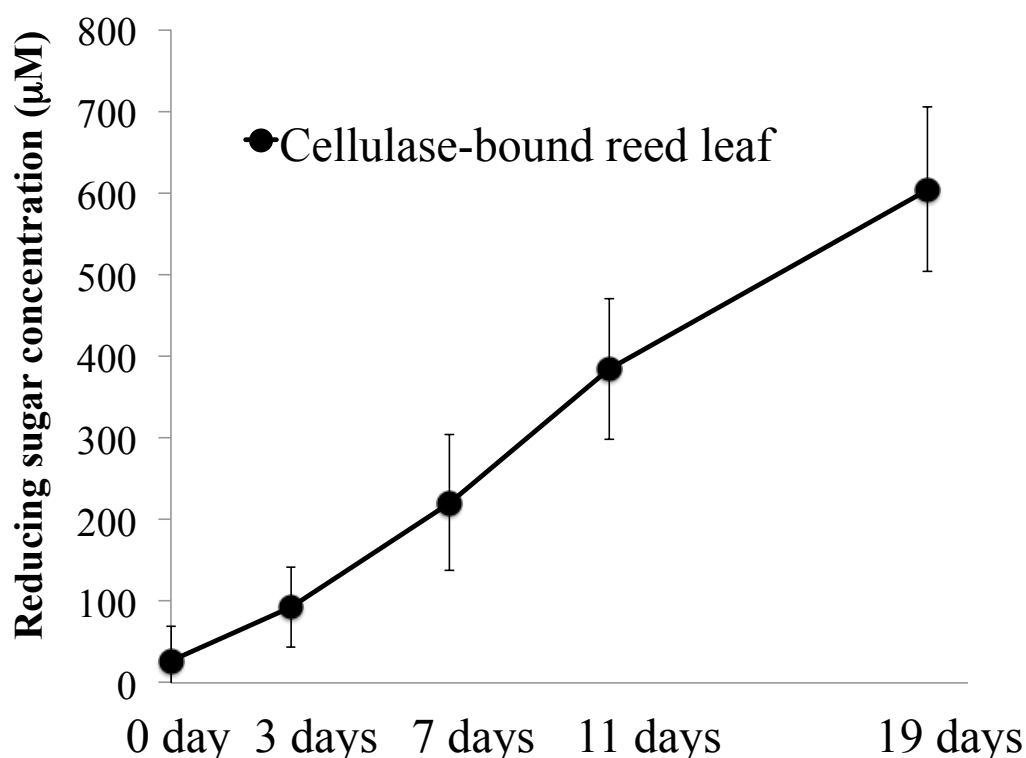
Fig.3-2-7 Reducing sugar production of the leaves collected in Fig.3-2-6 . Bars represent SEM (n = 3).
