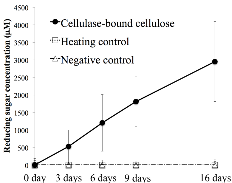
Fig.3-2-10 Reducing sugar production of the \alpha -cellulose collected in Fig.3-2-6 . Heating control, cellulose collected was heated at 100°C for 2 hours before the incubation. Negative control, cellulose without C. japonica culturing. All values are mean \pm SEM.
