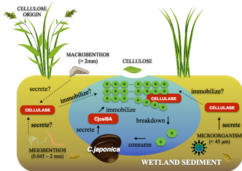
Fig. 3-2-21 “Environmental” cellulose decomposition system in wetland sediments. Scheme of the “environmental” cellulose decomposition system in wetland. Corbicula japonica exemplifies the bivalves that secrete cellulase to the environment. Secreted cellulase forms a immobilized complex. Cellulose is continually being decomposed into oligosaccharide and glucose. Glucose is consumed by C. japonica and amplifies its cellulase secretion. Other organisms are also considered to provide “environmental” cellulase (dotted arrows), making wetland a cellulose-decomposition factory.
