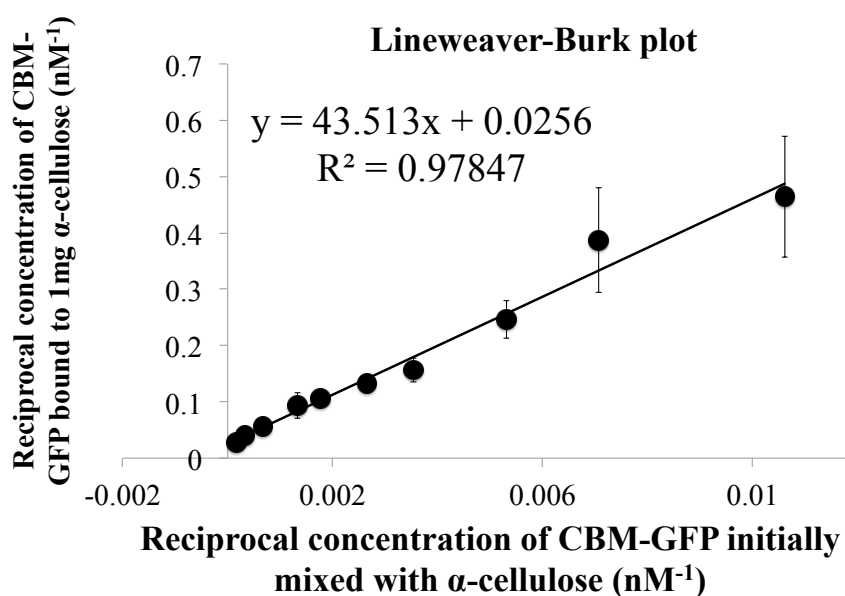
Fig.3-2-16 Lineweaver-Burk plot of Cjcel9A CBM against \alpha -cellulose.
