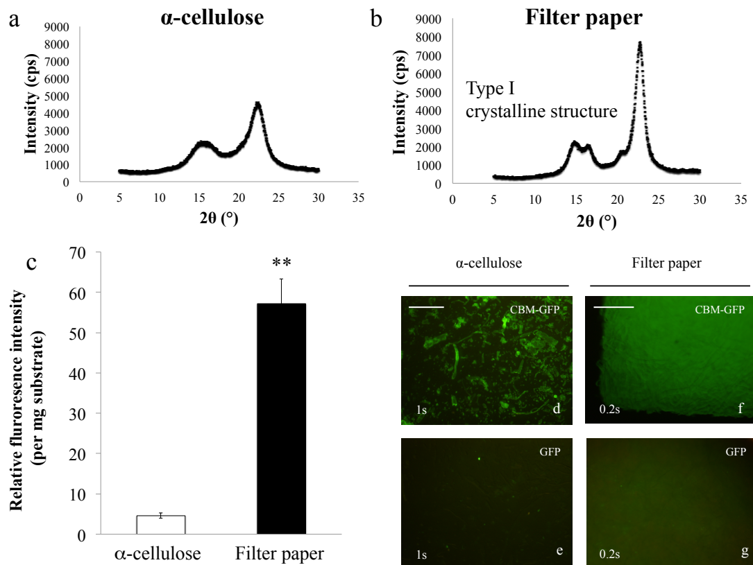
Fig. 3-2-18 Relationship between cellulose affinity and crystalline structure of cellulose. a, b , X-ray crystallographic assay of \alpha -cellulose ( a ) and filter paper ( b ). c , Affinity of Cjcel9A CBM for filter paper was significantly higher than that of \alpha -cellulose (**, P = 0.0000000612 , t -test). Values are mean \pm SEM. d, f , Fluorescence microscopy. e, g , GFP controls. Bottom left corners, exposure time. Exposure time (bottom left) and scale bars (left-up, 200 \mu m) are the same in the same column.
