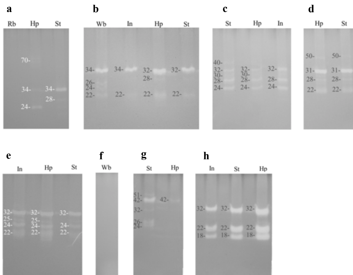
Fig. 1-6 Digestive organ distribution of mysid and decapod species by Zymographic assay. (a): Palaemon semmelinkii ; (b): Fenneropenaeus merguensis ; (c): Mierspenaeopsis sculptilis ; (d): Metapenaeus lysianssa ; (e): Metapenaeus ensis ; (f): Mesopodopsis tenuipes ; (g): Exopalaemon styliferus ; (h) Penaeus monodon . Abbreviated names of organs are shown on each sub-figure. Hp: hepatopancreas; St: Stomach; In: Intestine; Rb: rest of the body; Wb: whole body. Numbers the molecular sizes of each active band (kDa).
