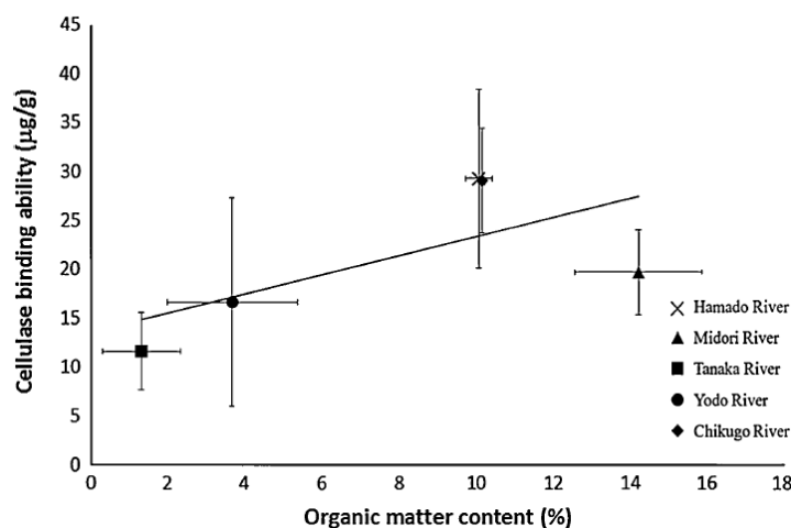
Fig. 3-1-1 Correlation between the organic matter content and the cellulase-binding ability of the sediments from various rivers. A strong correlation was demonstrated between them ( R = 0.66 )
