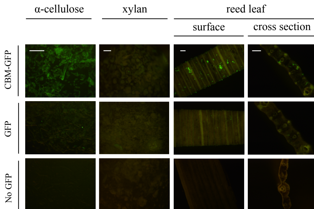
Fig. 3-2-15 Affinity of Cjcel9A CBM. Top panels, His 6 -CBM-GFP bound to \alpha -cellulose and reed leaves but not xylan. Middle panels, GFP controls. Bottom panels, autofluorescence controls. Exposure time, 1 s. Scale bars (upper left, 200 \mu m) shared in same column.
