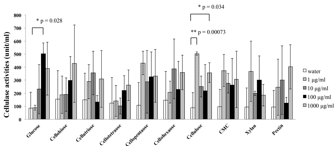
Fig. 3-2-19 Investigation of possible inducer that triggers cellulase secretion of C. japonica individuals. Glucose and cellulose triggered cellulase secretion. Values are mean \pm SEM.
