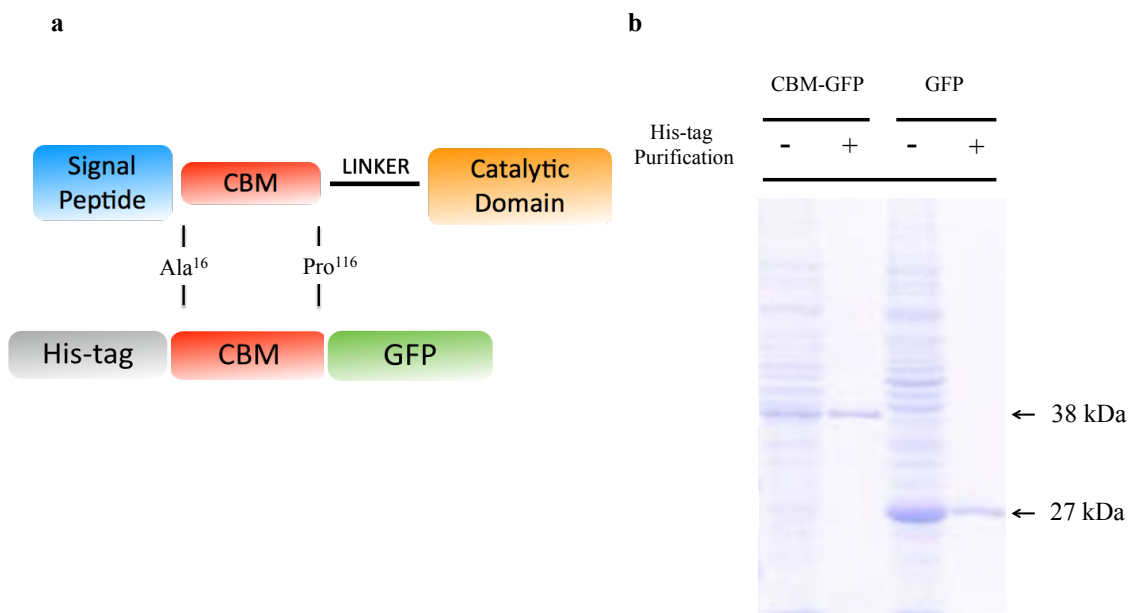
Fig. 3-2-14 Recombinant His 6 -CBM-GFP and His 6 -GFP expression and purification in XL-1 blue E. coli .
