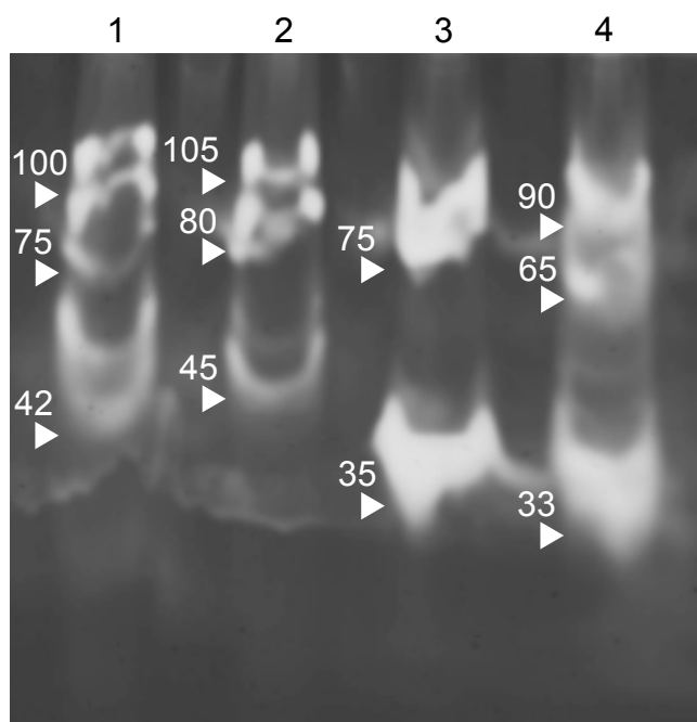
Fig. 2-3 Detection of deduced molecular weight of cellulases by using zymographic analysis. 1, Batillaria multiformis ; 2, B. attramentaria ; 3, Cerithidea cingulata ; 4, Cerithidea rhizophorarum . White triangle indicates the site of each band. Numbers denote the deduced molecular weight (kDa).
