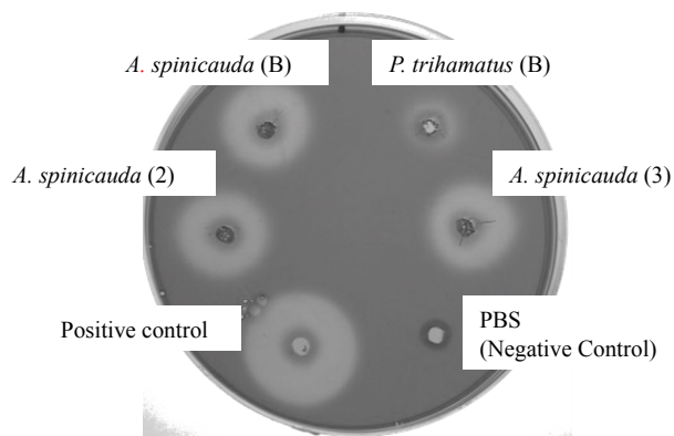
Fig. 1-2 Plate assays of copepod species in Selangor Estuary, Malaysia. Sampling sites are shown within parentheses. A positive control was prepared with commercially purchased cellulase.
