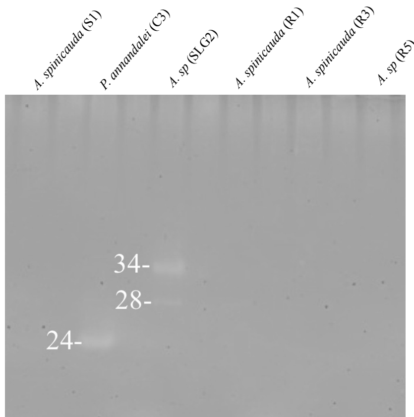
Fig. 1-5 Zymographic assay of copepod species in Matang Mangrove Forest Reserve, Malaysia. Inside the parentheses show the sampling sites, according to Table 1. Numbers show the molecular sizes of each active band (kDa).
