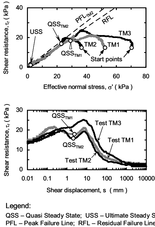
Fig. 4 Results of undrained monotonic ring shear tests on soil specimens from Tsukidate landslide
