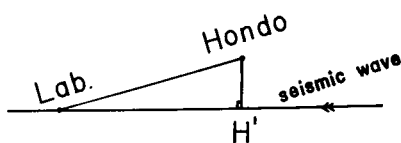
Fig. 6. Schematic illustration of the seismic path and stations.
