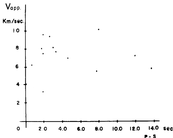
Fig. 12. Relation of the apparent velocity and P-S times for volcanic earthquakes.
