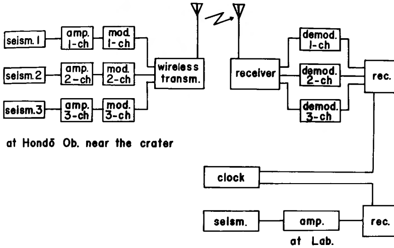
Fig. 2. Block diagram of telemetering system.
