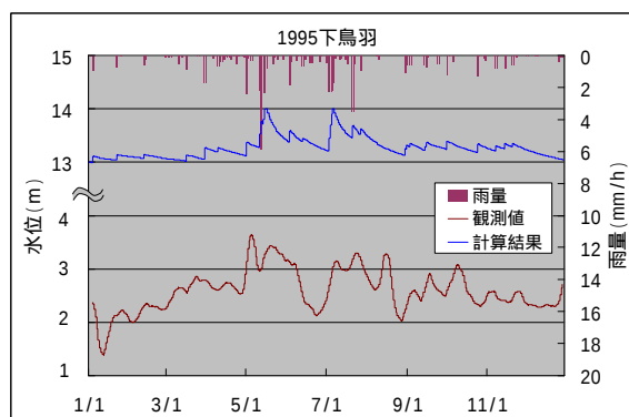
Fig.12 Calibration of groundwater level
