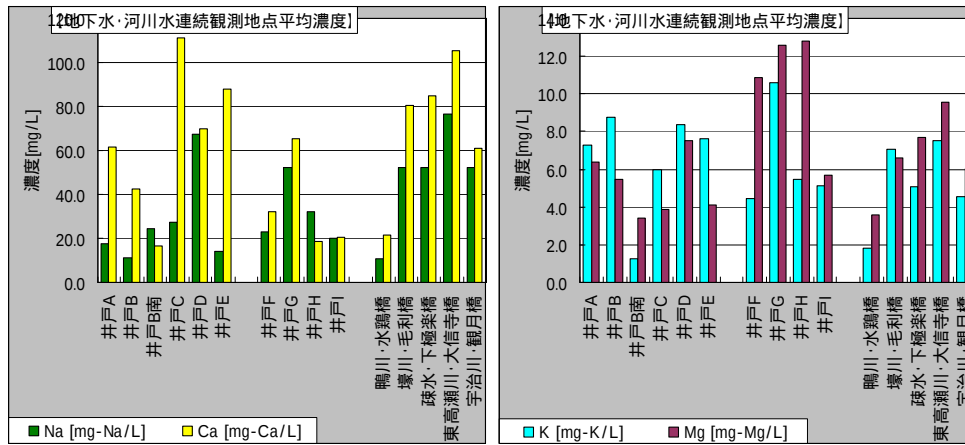
Fig.9 Kation concentration of observed well & river
