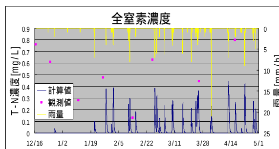
Fig.13 Simulation of groundwater quality
