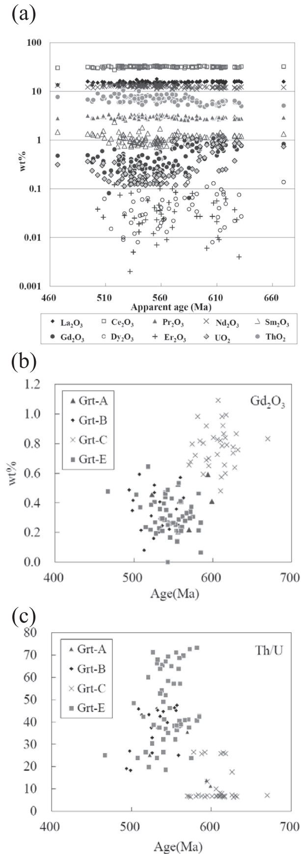
Figure 9. (a) REE, Th and U in monazite as a function of apparent U–Th–Pb monazite ages determined by the EMP. Note that the older monazite has higher \text{Gd}_2\text{O}_3 , \text{Sm}_2\text{O}_3 , and \text{UO}_2 contents, and lower \text{ThO}_2 content than the younger monazite. (b) A plot showing the correlation between \text{Gd}_2\text{O}_3 contents in monazite and apparent U–Th–Pb monazite ages. Note that the older monazite is richer in \text{Gd}_2\text{O}_3 . (c) A plot showing the correlation between the Th/U ratios of monazite vs apparent U–Th–Pb monazite ages. Note that the older monazite has low Th/U ratio. (b)–(c) ‘Garnet A’ represent monazite analyses from the grains (f) and (h) in Figure 8, ‘Garnet B’ represents those from the grains (a), (b), and (e), ‘Garnet C’ represents those from the grain (g), and ‘Garnet E’ represents those from the grains (c), (d), (i), and (j). Color version of Figure 9 is available online from http://doi.org/10.2465/jmps.150812 .
