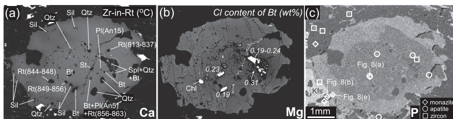
Figure 3. (a)–(c) X-ray elemental map of 'garnet B'. Other details are the same as Figures 2a–2c.
