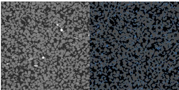
Point f (global degree of saturation=16.07%)
