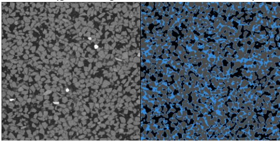
Point i (global degree of saturation=33.56%)
