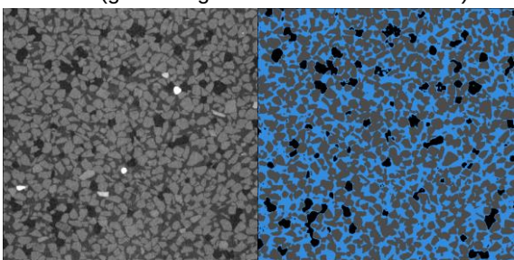
Point k (global degree of saturation=79.02%)
