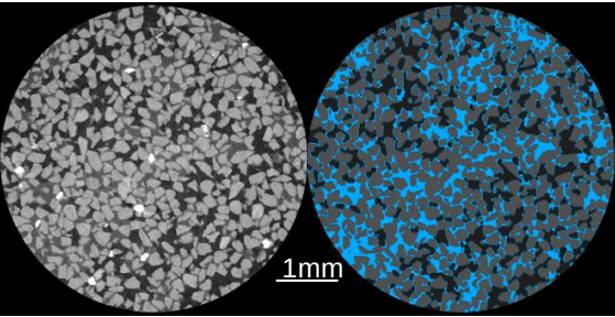
Point d (global degree of saturation=46.05%)
