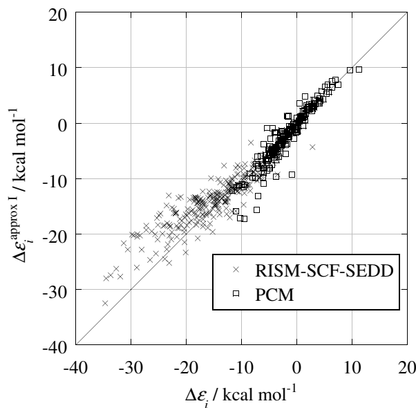
Figure 4.6: Comparison between the exact values ( \Delta\epsilon_i ) and the approximation formula of Eq. (4.15).
