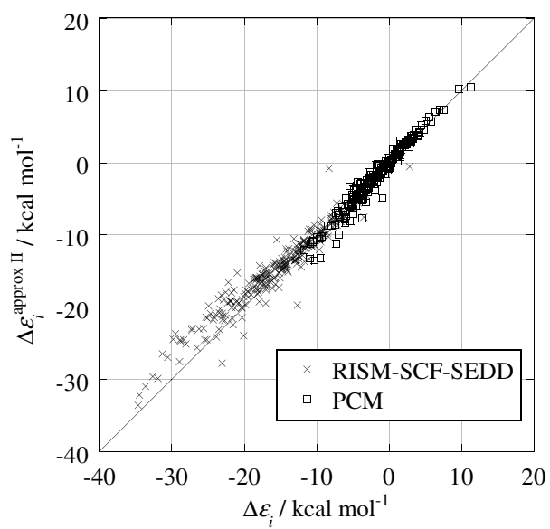
Figure 4.7: Comparison between the exact values ( \Delta\epsilon_i ) and the approximation formula of Eq. (4.16).
