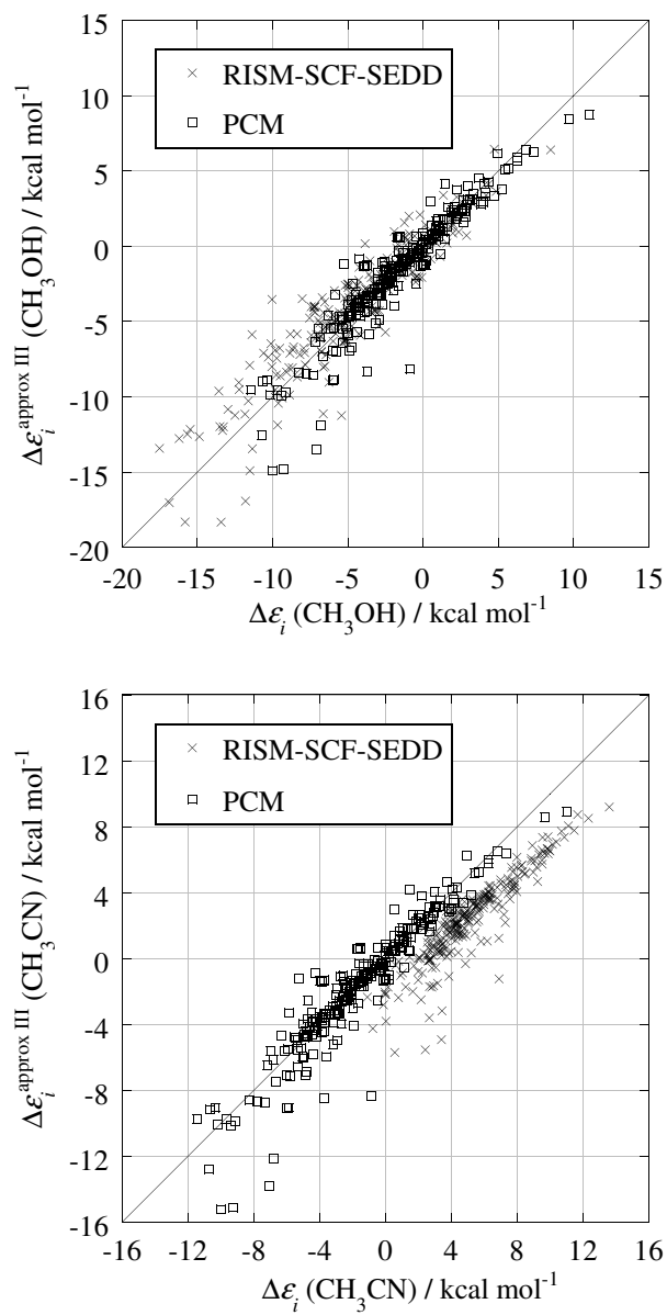
Figure 4.9: The energy shift in methanol (upper panel) and acetonitrile (lower panel). The exact values ( \Delta\epsilon_i ) and the approximation formula of Eq. (4.18) are compared.
