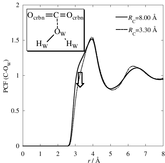
Figure 1.4: Pair correlation functions between C and O_W at R_C = 8.0 \text{ Å} (solid line) and R_C = 3.3 \text{ Å} (dotted line).
