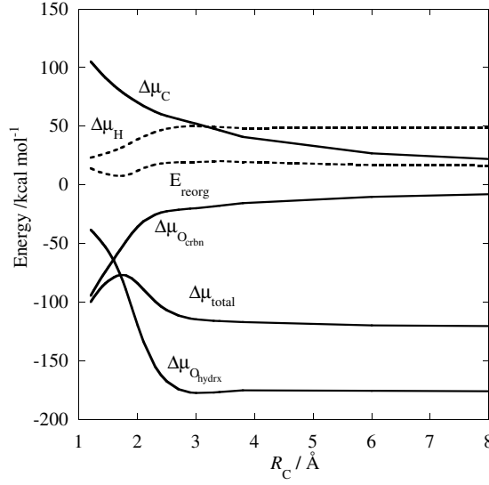
Figure 1.5: Electronic reorganization energy E_{\text{reorg}} , solvation free energy \Delta\mu and its components along the reaction coordinate.
