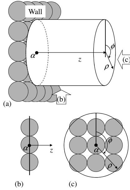
Figure 6.1: (a); Cylindrical coordinate system. (b); View from the direction perpendicular to z-axis. (c); View from the direction parallel to z-axis.
