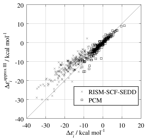
Figure 4.8: Comparison between the exact values ( \Delta\epsilon_i ) and the approximation formula of Eq. (4.18).
