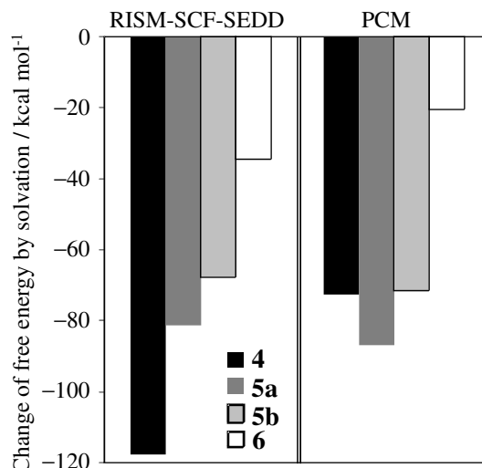
Figure 3.4: Change of free energy by solvation ( \Delta\mathcal{A} ) computed by RISM-SCF-SEDD (left) and PCM (right).
