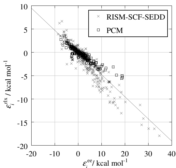
Figure 4.4: Comparison between \varepsilon_i^{\text{ee}} and \varepsilon_i^{\text{rlx}} , both of them are computed by PCM and RISM-SCF-SEDD. The slope of the plotted line is -0.476. See the text and Eq. (4.14).
