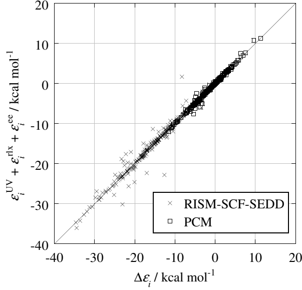
Figure 4.3: Comparison between the exact values ( \Delta\epsilon_i ) and Eq. (4.8)
