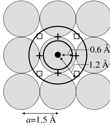
Figure 6.5: Relationship between the area from \rho = 0.6 \text{ \AA} to 1.2 \text{ \AA} and the molecular structure of the wall. \bullet : on-top position ( \rho = 0 \text{ \AA} ); + : bridge position ( \rho = a/2 ); \square : hollow position ( \rho = a/\sqrt{2} ).
