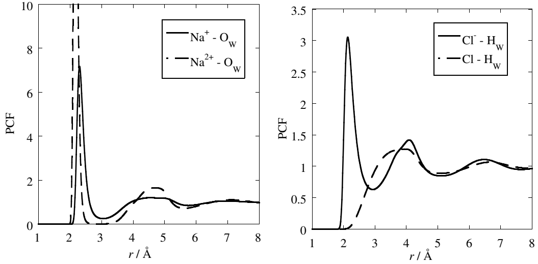
Figure 5.3: PCF between \text{Na}^+ and \text{O}_\text{W} , \text{Na}^{2+} and \text{O}_\text{W} (left hand panel), \text{Cl}^- and \text{H}_\text{W} , \text{Cl} and \text{H}_\text{W} (right hand panel) before ionization (solid line) and after ionization (dashed line).
