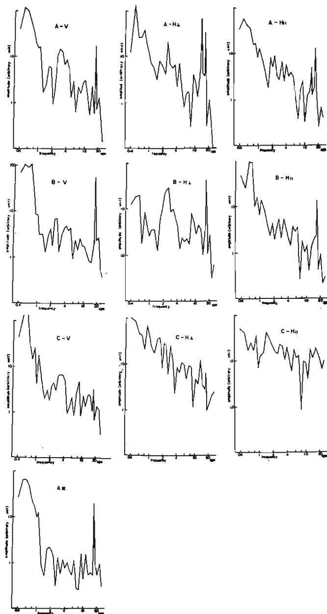
Fig. 4. Fourier amplitude spectrum of three components at A, B, C points and vertical component of St. point. H_{\perp} and H_{\parallel} show the horizontal components of setting up in the direction perpendicular and parallel to crack, respectively.
