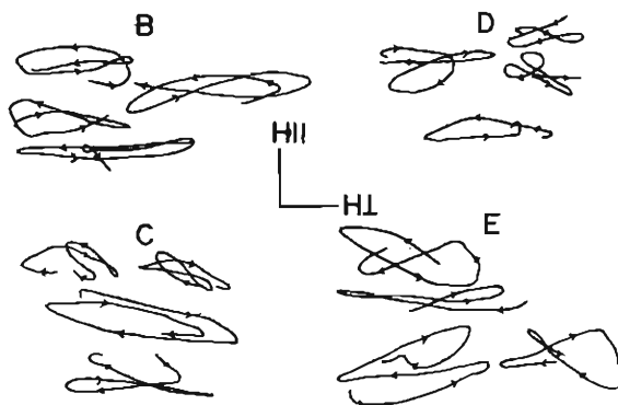
Fig. 6. Examples of particle motions of tremors in the frequency range from 2.5 to 6.3 Hz at B, C, D and E points.
