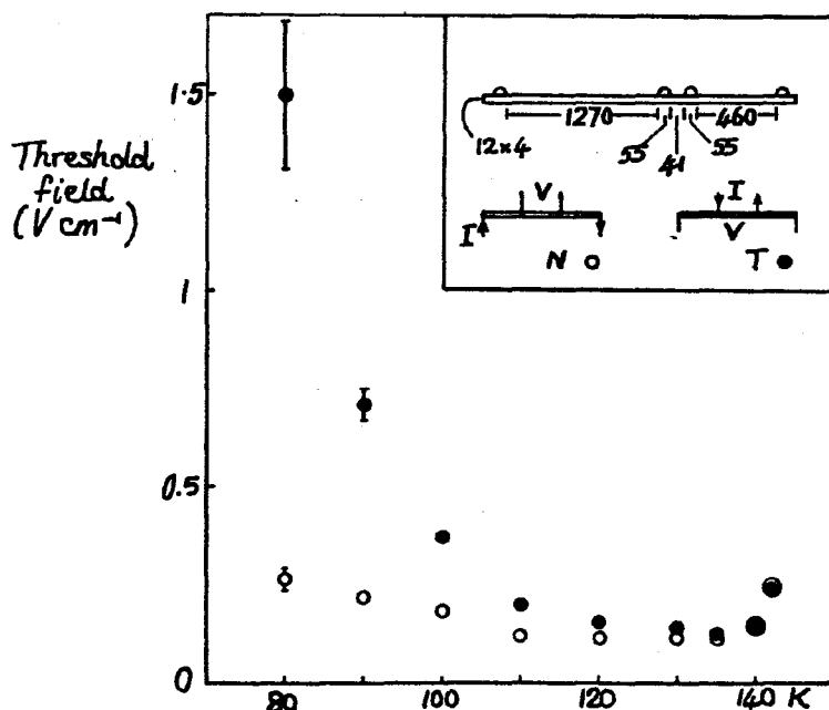
Figure 7. Apparent threshold fields measured in a \text{NbSe}_3 specimen using the normal (N; denoted \circ ) and transposed (T; denoted \bullet ) 4-terminal configurations. These arrangements, and the dimensions of the specimen (in \mu\text{m} ) are shown inset.
