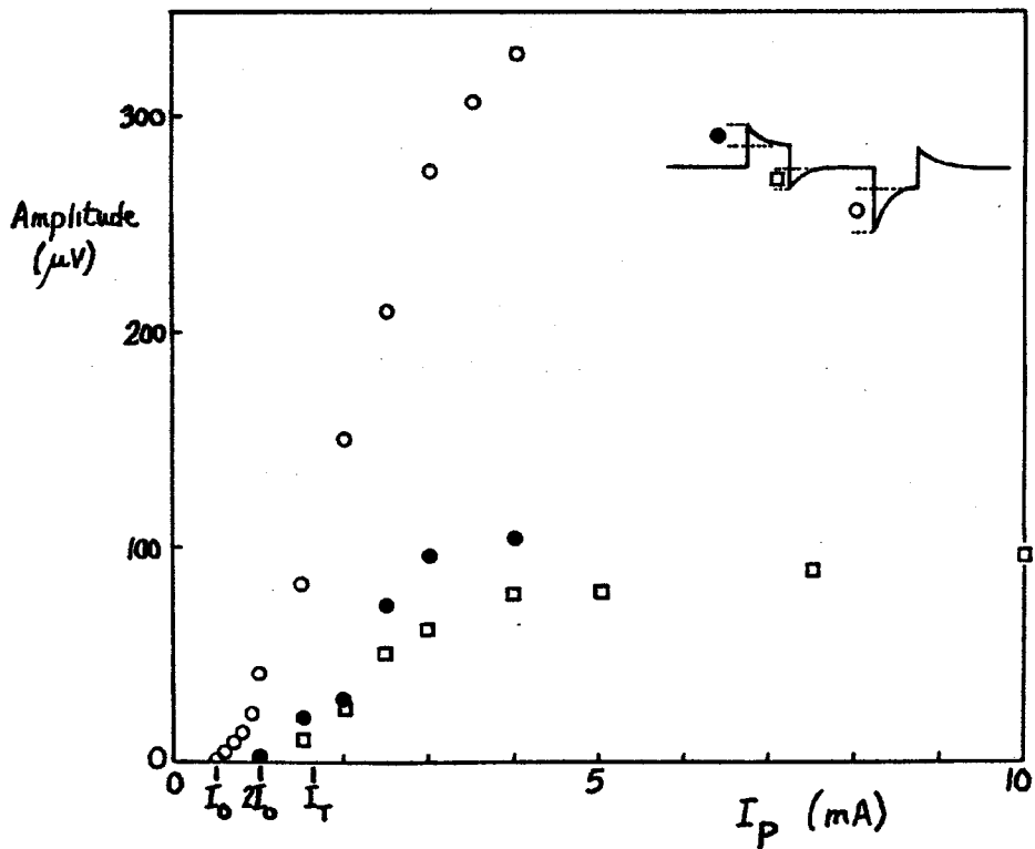
Figure 9. The dependence of the amplitudes of the reversal (o), relaxation (□) and re-establishment (●) transients on the amplitude I_p of the current pulses. The threshold currents predicted by the simple model are also indicated.
