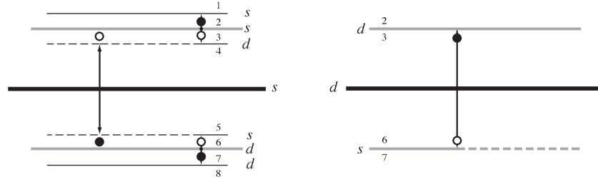
Figure 5. The diagram representing the multiple crossing on the real axis for the n = 3 case. The diagram for \operatorname{Re} q_{n+1} < 0 (left) and for \operatorname{Re} q_{n+1} > 0 (right).
