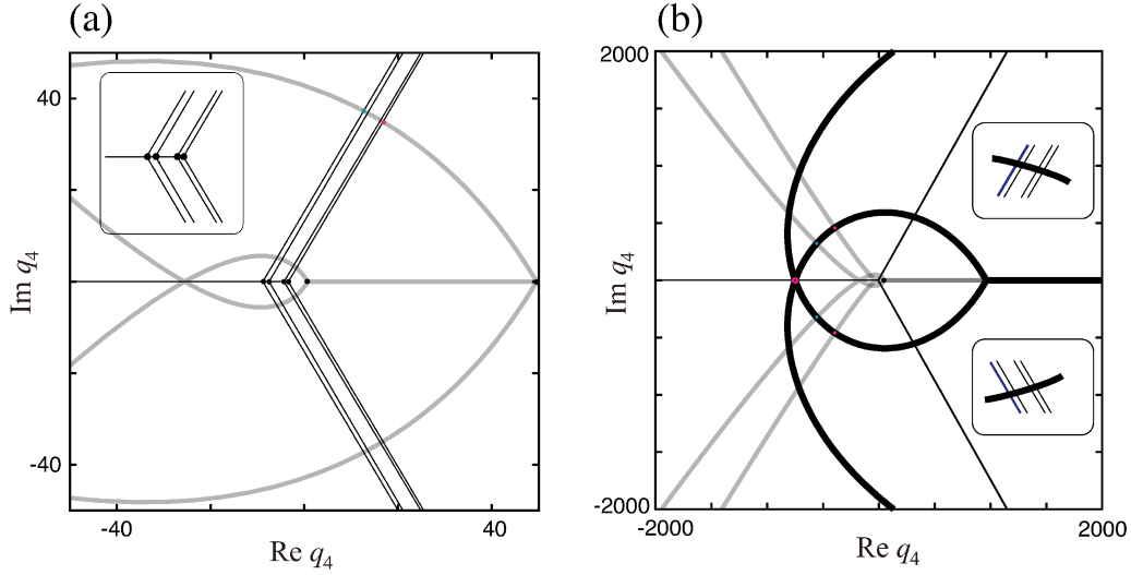
Figure 1. The ordinary Stokes curves for n = 3 with the values of parameters c = -6.0 and q_0 = 0 . The bold, gray and thin curves are Stokes curves for the 1st, 2nd and 3rd generation, respectively (see text). The inset in (a) shows the magnification around the ordinary turning points for the 3rd generation and that in (b) indicates the crossing points between the Stokes curves for the 1st and 3rd generation outside the range of this scale.
