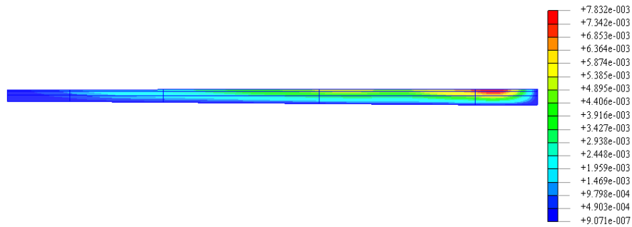
Fig.14 Ground strain distribution in the axial direction in the case4-1
