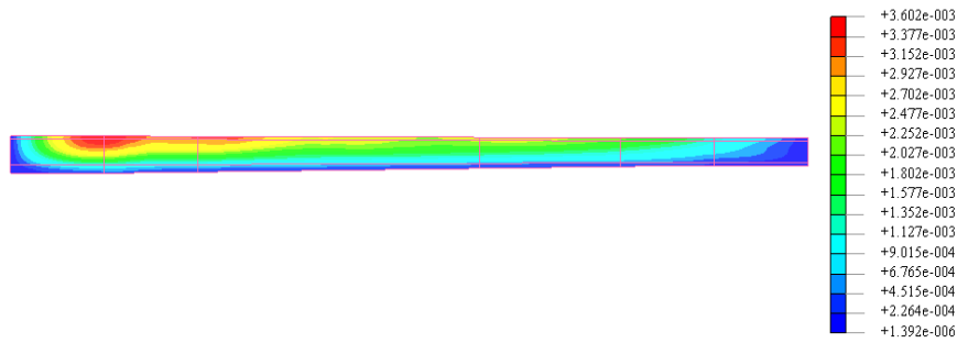
Fig.13 Ground strain distribution in the axial direction in the case3-1
