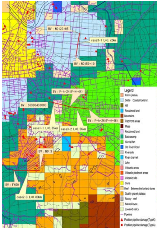
Fig.3 A damage position and analysis position in Kashiwazaki city center
