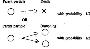
Fig 1 Binary Branching
