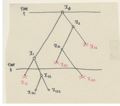
Figure 2 Example of a Realized Tree \omega_1
