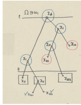
Figure 3 Classification of Nodes for \omega_1
