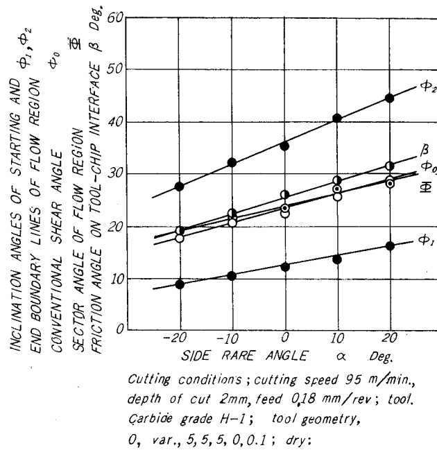
Fig. 5 (a). Calculation value of grey cast iron with side rake angle.
