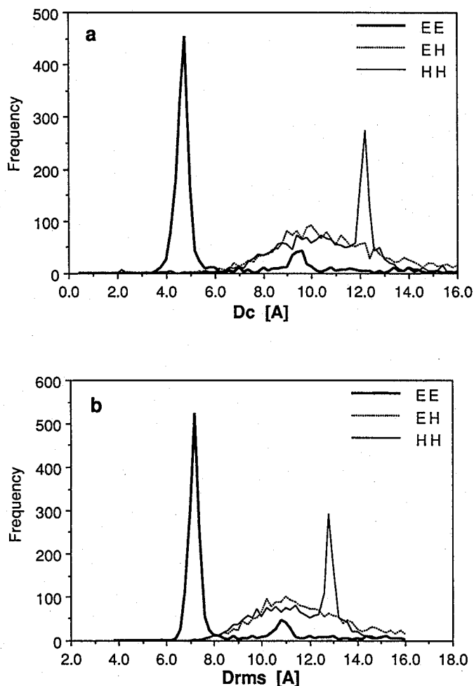
Fig. 3 The observed frequencies of segment-pairs in 'EE', 'EH', and 'HH' groups plotted against the distance in (a) Dc and in (b) Drms. The segment length was: L = 4 . 'EE', thick solid line; 'EH', dotted line; and 'HH', thin solid line.
