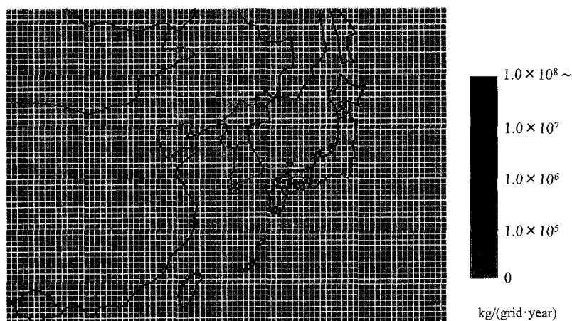
Fig. 2. Sulfur dioxide emission with 60 km×60 km grid resolution (1995).
