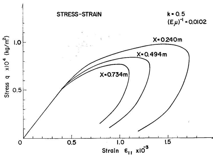
Fig. 10 Stress-strain relationship.
