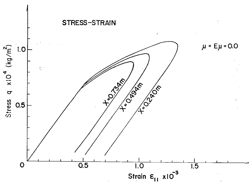
Fig. 13 Stress-strain relationship.
