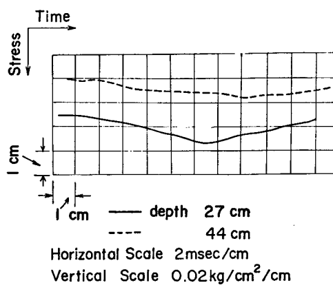
Fig. 2 Pore pressure-time profile.
