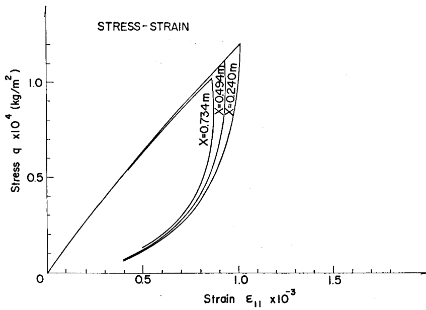
Fig. 15 Stress-strain relationship.
