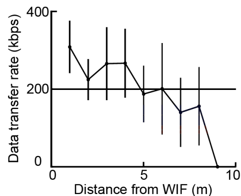
Fig. 6 | Decreased rates of data transmission across far distances.
