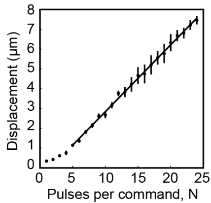
Fig. 4 | Electrode displacement as a function of pulse number. Plot showing that the displacement of an electrode is a linear function of a number of pulses within 5 to 24 pulses (displacement (μm) = 0.338N - 0.54 for N \geq 5 with R^2 = 0.997 ). Vertical line indicates s.e.m.; n = 10 .
