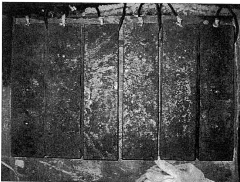
Figure 4.13 Corrosion of steel plate bonded on concrete specimen
