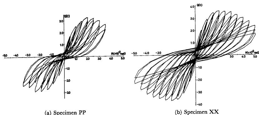
Fig. 8. Load-Deflection Relationships
