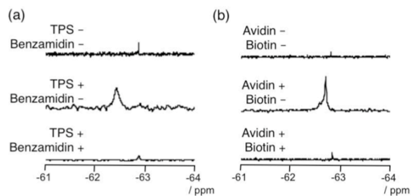
Figure 3. Turn-on ^{19}\text{F} NMR detection of trypsin and avidin by probe 3 and 5 . (a) ^{19}\text{F} NMR spectra of 3 (100 \mu\text{M} ) in the absence or presence of TPS (50 \mu\text{M} ) and benzamidine (500 \mu\text{M} ) in 50 mM Tris-HCl buffer (pH 8.5, 0.2 mM TFA, 300 mM NaCl, 10% \text{D}_2\text{O} (v/v)). The SNR was 12.2. (b) ^{19}\text{F} NMR spectra of 5 (100 \mu\text{M} ) in the absence or presence of avidin (50 \mu\text{M} ) and biotin (500 \mu\text{M} ) in 50 mM HEPES buffer (pH 7.2, 0.2 mM TFA, 500 mM NaCl, 10% \text{D}_2\text{O} (v/v)). The SNR was 57.3.
