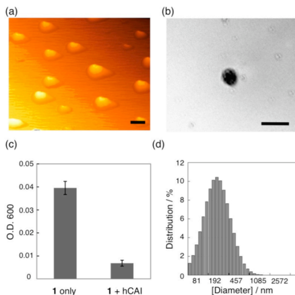
Figure 2. Microscopic and spectroscopic characterization of the self-assembled nano-particles of probe 1 . (a) AFM image of the self-assembled probe 1 (25 \mu M). The scale bar is 500 nm. (b) TEM image of the self-assembled probe 1 (25 \mu M). The scale bar is 500 nm. (c) Optical density at 600 nm of aqueous solution containing probe 1 (25 \mu M) in the absence (left) or presence (right) of hCAI (25 \mu M). Experiments were performed in triplicate to obtain mean and standard deviation values (shown as error bars). (d) DLS analysis of particle size distribution of the self-assembled probe 1 (25 \mu M). All experiments were performed in 50 mM HEPES buffer (pH 7.2, 0.2 mM TFA).
