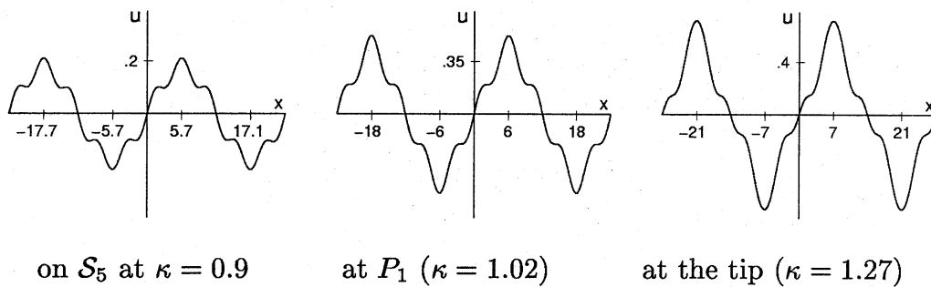
Fig. 4.2a. The first three solutions
