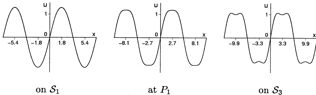
Fig. 4.4. Three solutions on the branch in Figure 4.3
