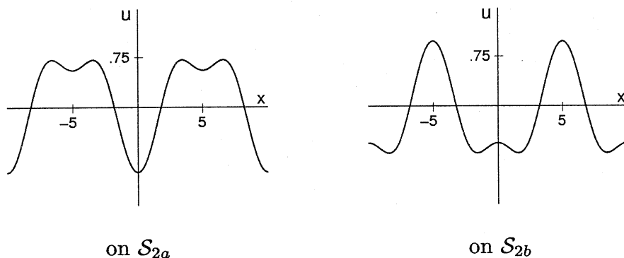
Fig. 2.5. Solutions of Theorem 2.4
