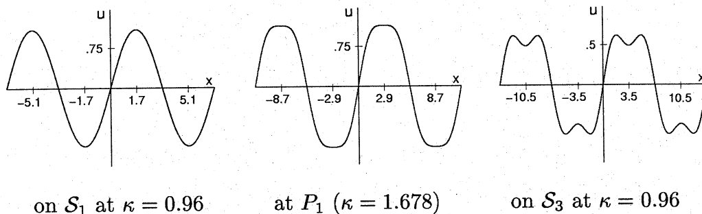
Fig. 2.2. Solution graphs on the loop shown in Figure 2.1
