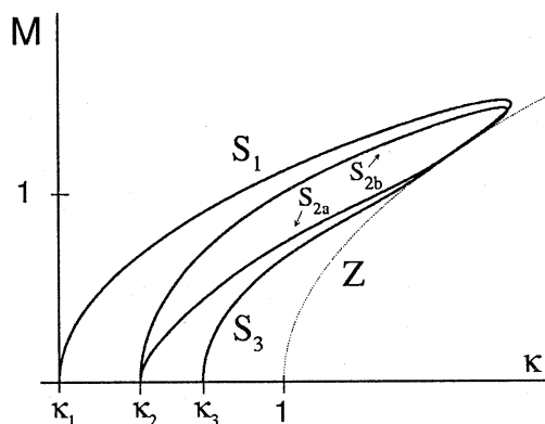
Fig. 2.4. The branches S_1 , S_{2a} , S_{2b} and S_3
