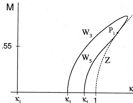
Fig. 2.7. The branches \mathcal{W}_3 and \mathcal{W}_5
