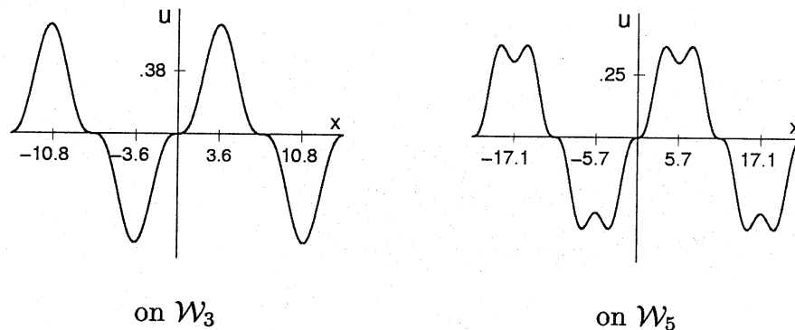
Fig. 2.6. Solutions on branches \mathcal{W}_3 and \mathcal{W}_5 at \kappa = .96
