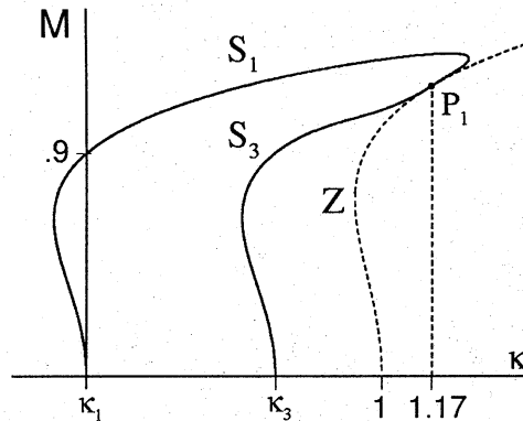
Fig. 4.3. The branches \mathcal{S}_1 and \mathcal{S}_3 , and the graph of Z
