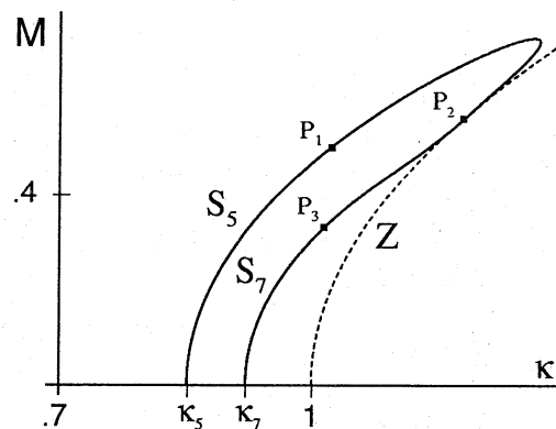
Fig. 4.1. The branches S_5 and S_7
