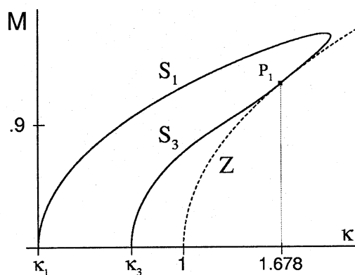
Fig. 2.1. The branch \mathcal{S}_1 of odd 1-Lap periodic solutions and the branch \mathcal{S}_3 of odd 3-Lap solutions
