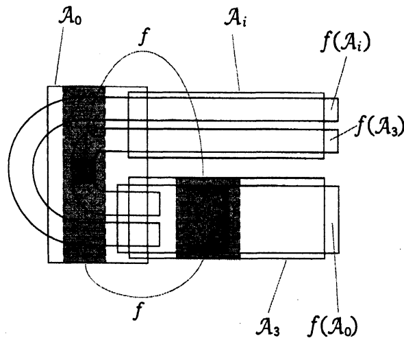
Figure 1. Poincaré boxes for the cubic Hénon map f_{a,b} .
