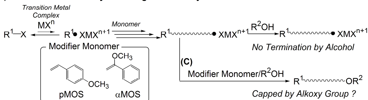
Scheme 1. Quantitative End-Capping with Alcohols in Living Polymerization
