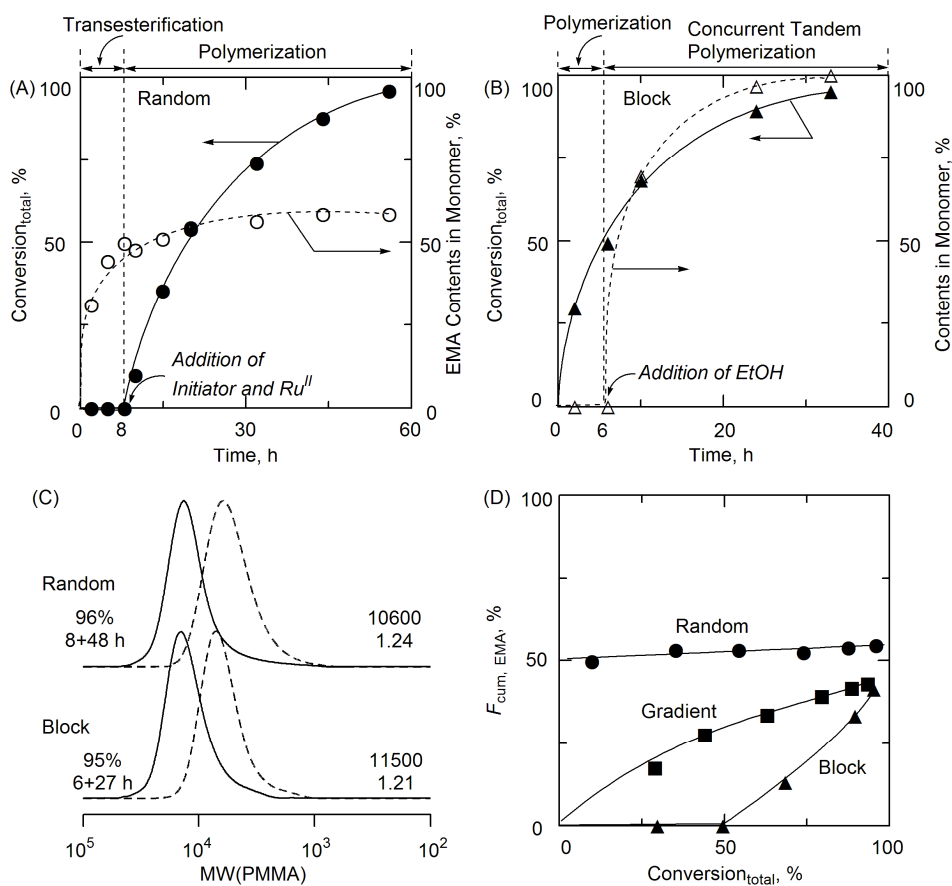
Figure 10. Effects of initiation timing of transesterification and polymerization in tandem living radical polymerization: (A), (B) total conversion and EMA contents in polymerization solution, (C) SEC curves of products, (D) cumulative EMA contents in products ( F_{\text{cum, EMA}} ) as a function of total conversion. Gradient: the same samples as the product with \text{Al}(\text{O}i\text{-Pr})_3 in Figure 4. Random: [\text{MMA}]_0 = 2.0 \text{ M} ; [\text{Ti}(\text{O}i\text{-Pr})_4]_0 = 20 \text{ mM} ; [\text{EtOH}]_0 = 2.0 \text{ M} ; [\text{ECPA}]_{\text{add}} = 20 \text{ mM} ; [\text{Ru}(\text{Ind})\text{Cl}(\text{PPh}_3)_2]_{\text{add}} = 2.0 \text{ mM} in toluene at 80^\circ\text{C} . Block: [\text{MMA}]_0 = 2.0 \text{ M} ; [\text{ECPA}]_0 = 20 \text{ mM} ; [\text{Ru}(\text{Ind})\text{Cl}(\text{PPh}_3)_2]_0 = 2.0 \text{ mM} ; [\text{Ti}(\text{O}i\text{-Pr})_4]_0 = 20 \text{ mM} ; [\text{EtOH}]_{\text{add}} = 6.5 \text{ M} in toluene at 80^\circ\text{C} .
