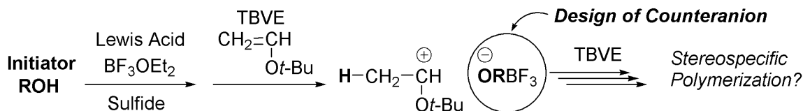
Scheme 1. Design of Counteranion with Alcohols toward Stereospecific Polymerization
