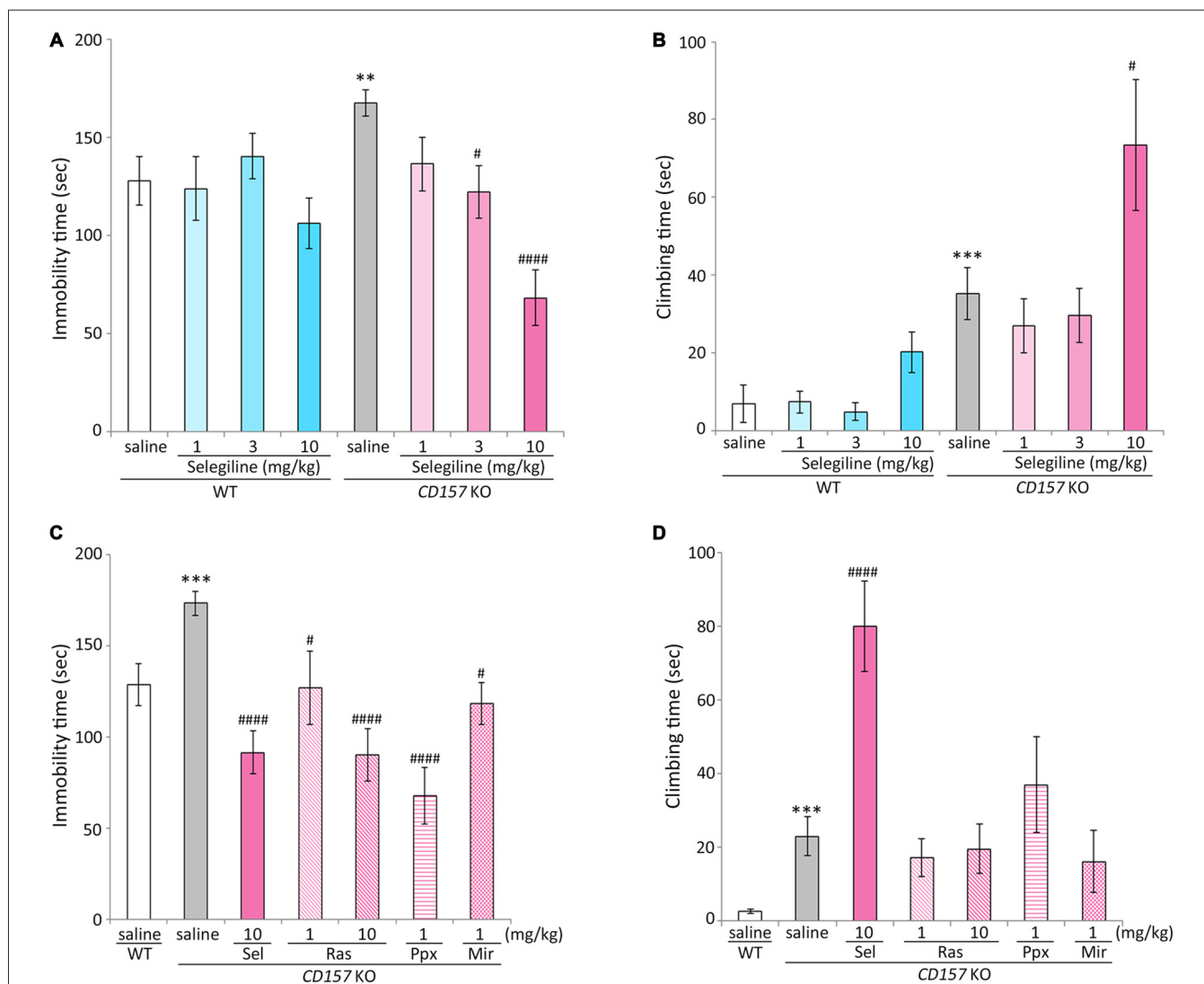
FIGURE 1 | Effects of monoamine oxidase-B (MAO-B) inhibitors, a dopamine (DA) agonist and a noradrenergic and specific serotonergic antidepressant (NaSSA) on a depression-like behavior in CD157/BST1 knockout ( CD157 KO ) mice subjected to the forced swimming test (FST). (A) A single administration of selegiline (1–10 mg/kg, subcutaneous, s.c.) reduced immobility time of CD157 KO mice in the FST. ** P < 0.01 , saline-treated CD157 KO mice vs. saline-treated wild-type (WT) mice (Student's t -test), # P < 0.05 , #### P < 0.001 vs. saline-treated CD157 KO mice (Dunnett's test), F_{(3,64)} = 12.539 , P < 0.001 . A two-way analysis of variance (ANOVA) showed a significant interaction between the effects of treatment and genotypes on the immobility time ( F_{(3,128)} = 3.904 , P < 0.05 ). (B) A single s.c. administration of selegiline at 10 mg/kg, but not 3 mg/kg, significantly increased climbing time of CD157 KO mice. The data are expressed as the mean \pm SEM ( n = 21 –22 for saline-treated WT and CD157 KO mice, n = 15 –17 for selegiline-treated WT and CD157 KO mice). *** P < 0.005 , saline-treated CD157 KO mice vs. saline-treated WT mice (Student's t -test), # P < 0.05 vs. saline-treated CD157 KO mice (Dunnett's test), F_{(3,67)} = 4.382 , P < 0.01 . A two-way ANOVA showed no significant interaction between the effects of treatment and genotypes on the climbing time ( F_{(3,131)} = 1.684 , P = 0.174 ). (C) A single administration of selegiline (Sel; 10 mg/kg, s.c.), rasagiline (Ras; 1, 10 mg/kg, s.c.), or pramipexole (Ppx; 1 mg/kg, s.c.) and repeated administration of mirtazapine (Mir; 1 mg/kg, intraperitoneally, i.p.) reduced immobility time of CD157 KO mice in the FST. *** P < 0.005 , saline-treated CD157 KO mice vs. saline-treated WT mice (Student's t -test), # P < 0.05 , #### P < 0.001 vs. saline-treated CD157 KO mice (Dunnett's test), F_{(5,86)} = 10.276 , P < 0.001 . (D) Selegiline (10 mg/kg, s.c.) increased the climbing time of CD157 KO mice, but rasagiline, pramipexole and mirtazapine did not. Data are expressed as mean \pm SEM ( n = 22 –24 for saline-treated WT and CD157 KO mice, n = 12 –19 for drug-treated CD157 KO mice). *** P < 0.005 , saline-treated CD157 KO mice vs. saline-treated WT mice (Student's t -test), #### P < 0.001 vs. saline-treated CD157 KO mice (Dunnett's test), F_{(5,87)} = 8.471 , P < 0.001 .
