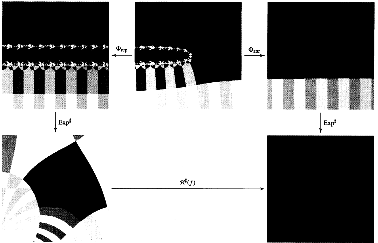
FIGURE 1. Parabolic renormalization \mathcal{R}^\sharp(f) for \eta = 2 . Since e^{4\pi} \approx 286751 is too large, some parts in the renormalized pictures are too large or too small to see.
