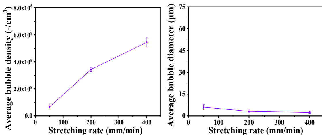
Figure S11. Bubble density and diameter of the stretching-induced SIBS073T-N 2 foams prepared with 4 MPa N 2 at different stretching rates (300% strain).
