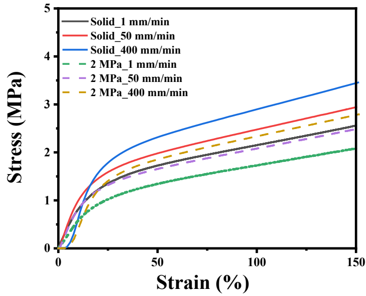
Figure S6. S-S curves of solid SIBS073T and CO 2 -laden SIBS073T samples (2 MPa).
