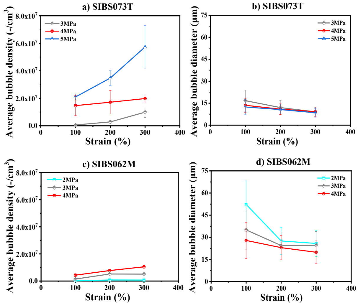
Figure 8. Bubble densities and diameters of stretching-induced foams of SIBS073T (a, b) and SIBS062M (c, d) at three different strains with a 400 mm/min stretching rate.
