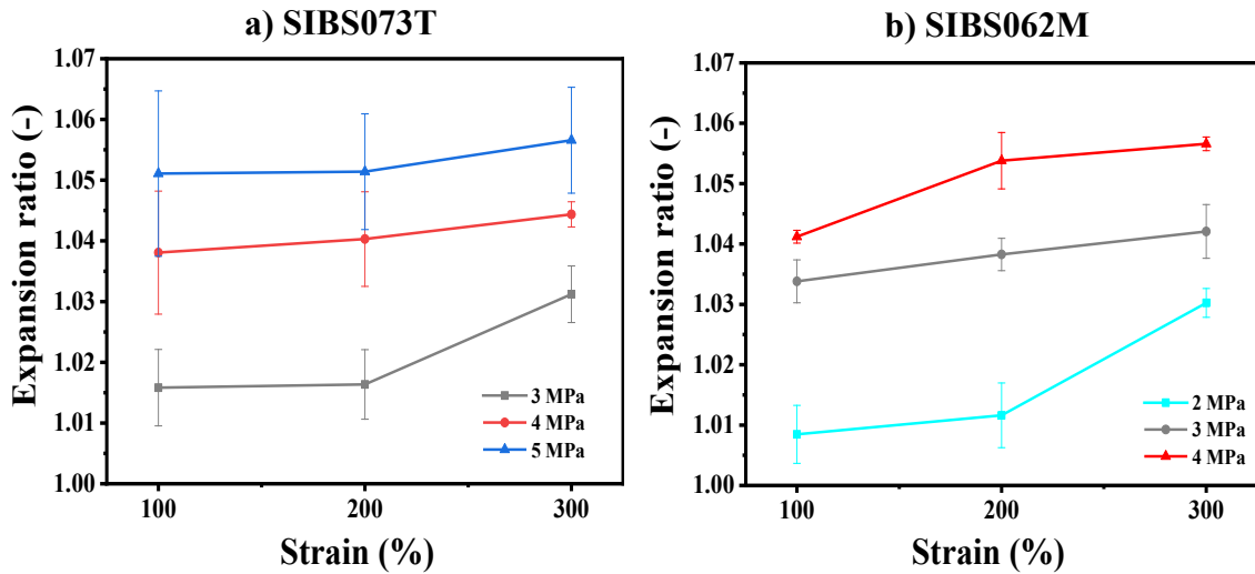
Figure S9. Expansion ratio of the SIBS073T and 062M stretching-induced foams.
