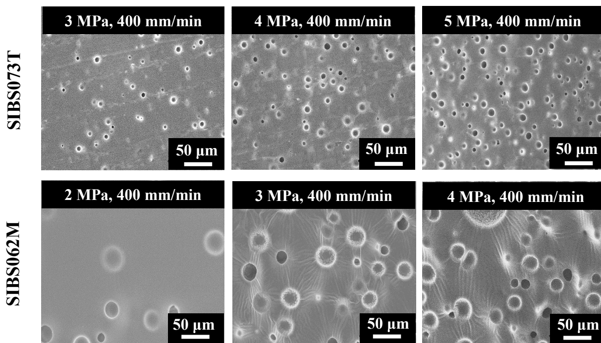
Figure 5. SEM images of the stretching-induced foams of SIBS073T and 062M with various pressures.
