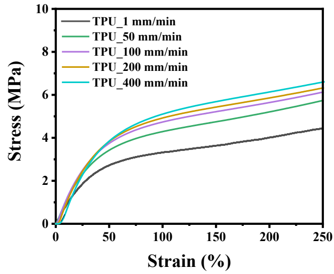
Figure S16. Strain–stress (S–S) curves of quasi-static and dynamic tests of TPU solid samples.
