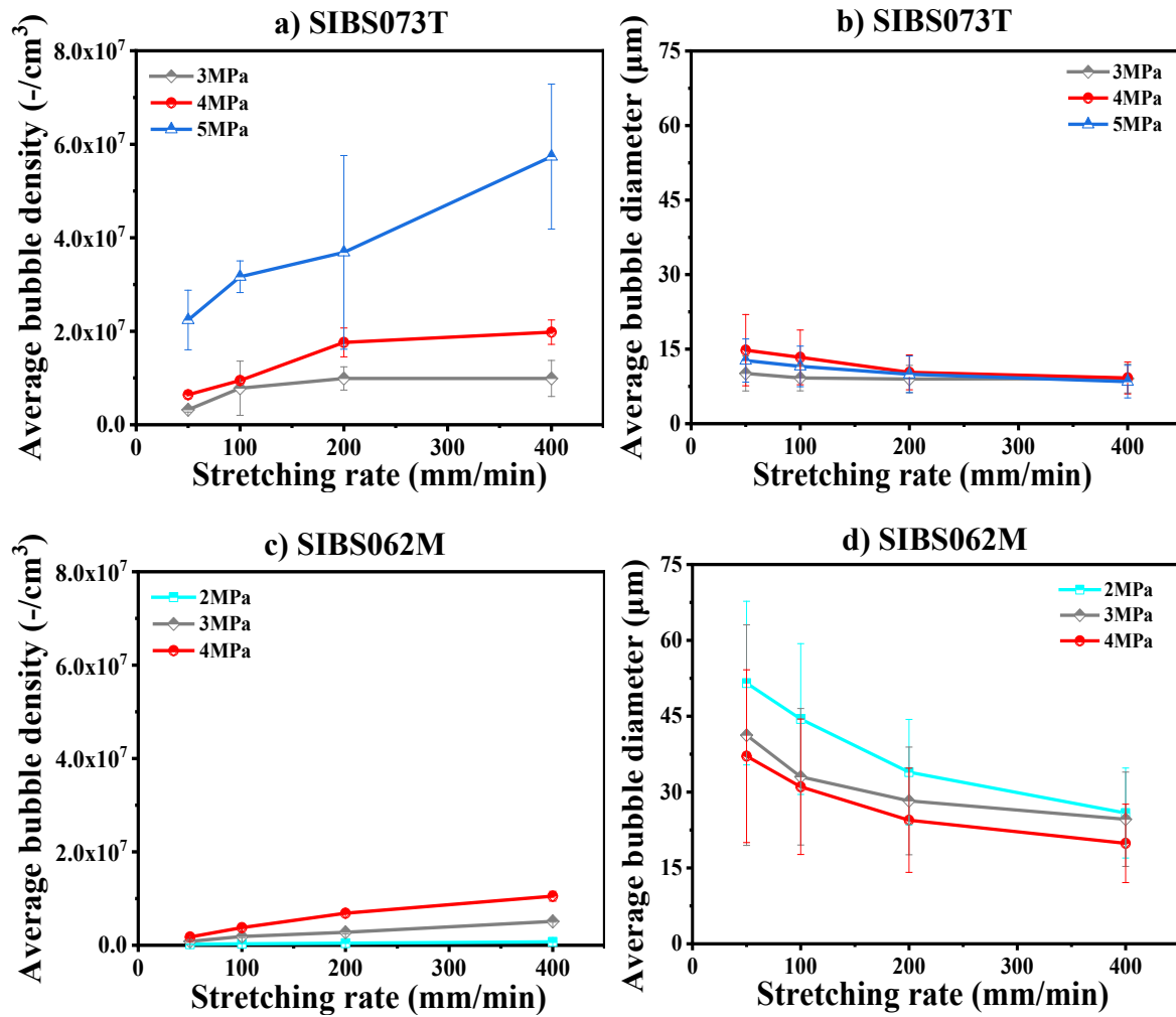
Figure 7. Bubble densities and diameters of stretching-induced SIBS073T (a, b) and SIBS062M (c, d) foams prepared at different stretching rates with 300% strain.
