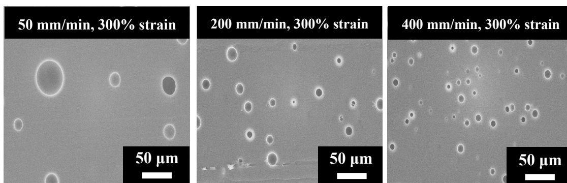
Figure S12. SEM images of the stretching-induced N_2 -laden TPU at different stretching rates (0, 50, 200, and 400 mm/s)
