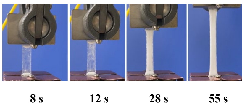
Figure 3. A series of snapshots of stretching-induced foaming at 50 mm/min stretching rate with 300% final strain (gas delivery pressure: 5 MPa).
