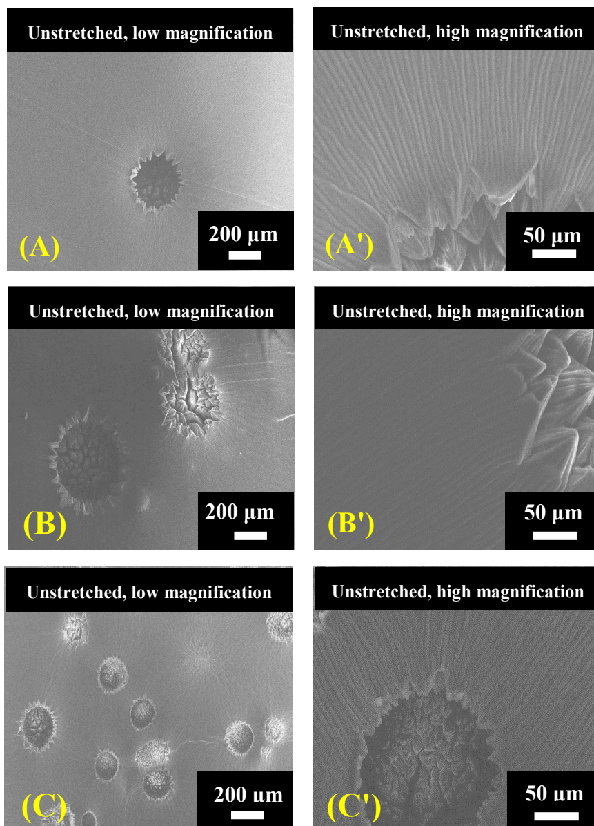
Figure S8 SEM images of unstretched CO 2 -laden SIBS062M samples with different CO 2 delivery pressures: (A)-(C) are low magnification images and (A')-(C') are high magnification: ((A) and (A'): 3MPa, (B) and (B'): 4MPa, (C) and (C'): 5MPa)
