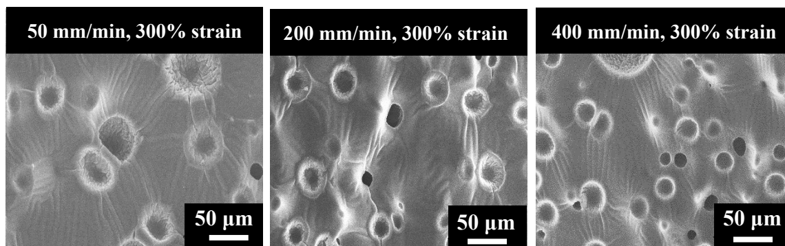
Figure S3. SEM images of cell structure of the stretching-induced foams of SIBS062M at different stretching rates (50, 200 and 400 mm/min) with strain of 300% and 5 MPa delivery pressure.
