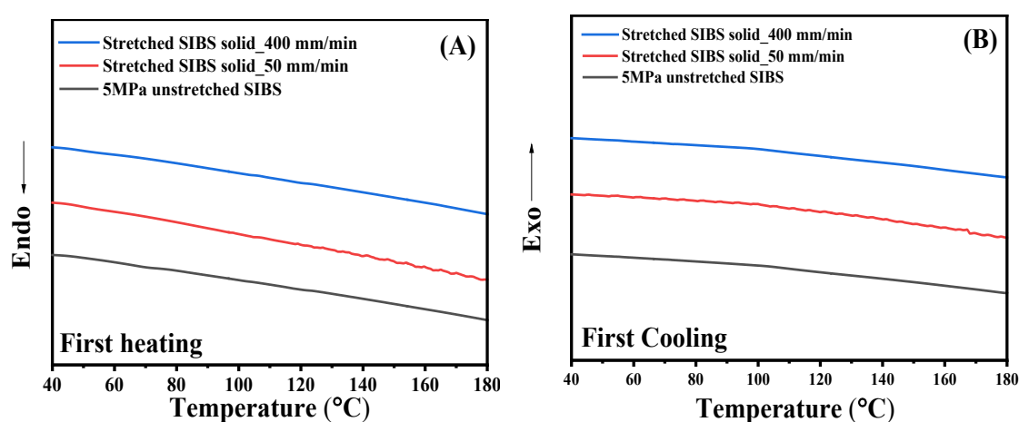
Figure S17. First heating curves and cooling curves of stretched SIBS073T samples: stretched solid samples with stretching rates of 50 and 400 mm/min, and unstretched sample (5 MPa).
