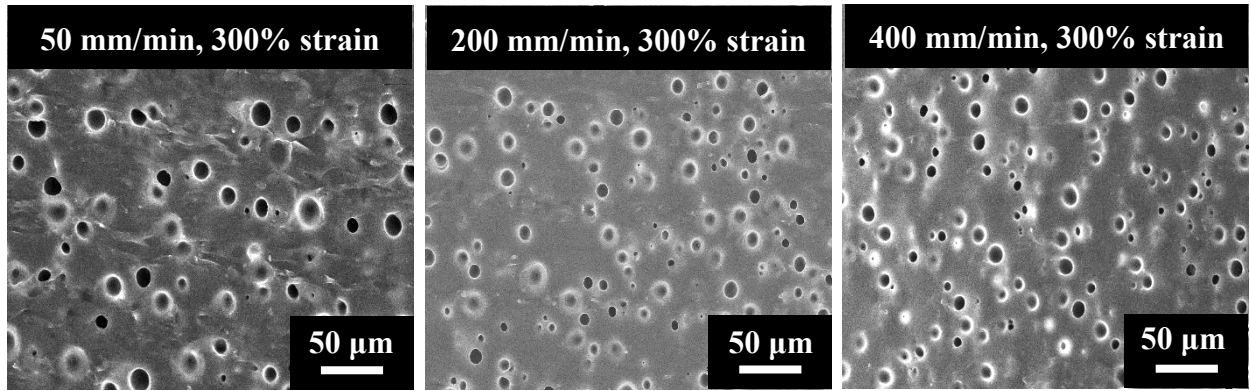
Figure 6. SEM images of the cell structure of stretching-induced foams of SIBS073T at different stretching rates (50, 200 and 400 mm/min) with strains of 300% and 5 MPa delivery pressure.
