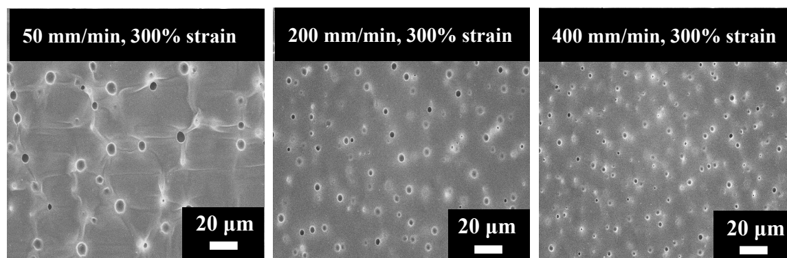
Figure S10 SEM images of the stretching-induced N 2 -laden SIBS products at different stretching rates (0, 50, 200, and 400 mm/s)
