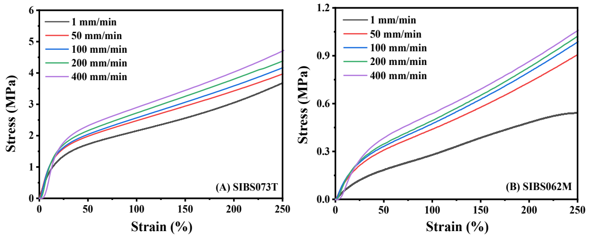
Figure 1. Strain–stress (S–S) curves of quasi-static and dynamic tests of solid samples. (A): SIBS073T and (B): SIBS062M.
