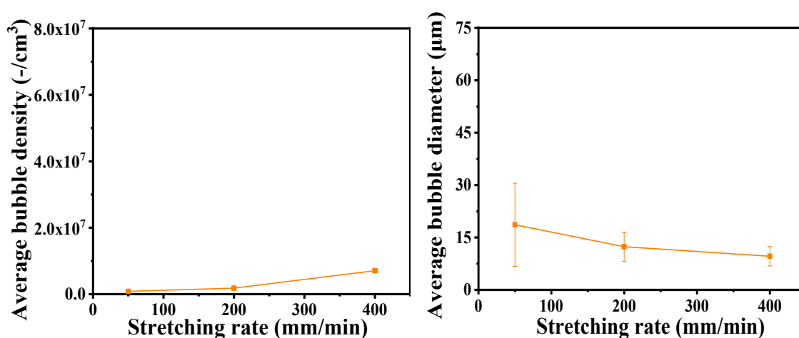
Figure S13. Bubble density and diameter of the stretching-induced TPU foams prepared with 5 MPa N_2 at different stretching rates (300% strain).
