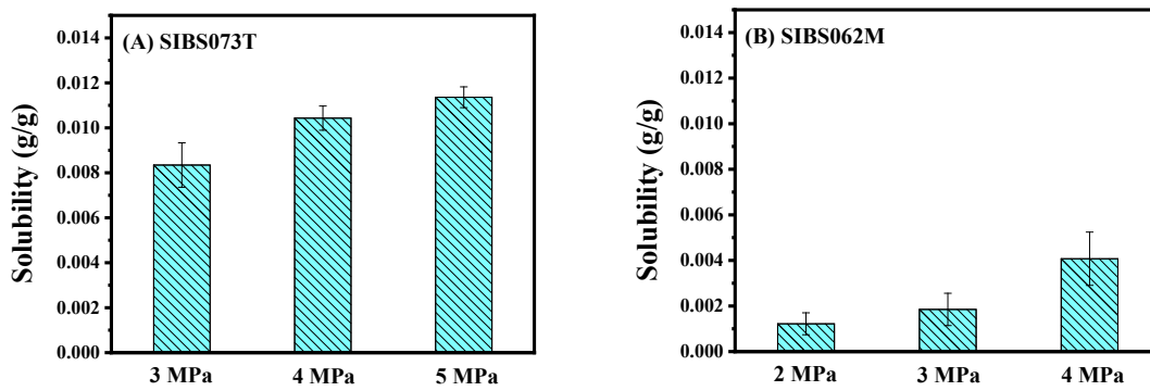
Figure 4. CO 2 contents in SIBS before stretching at room temperature.
