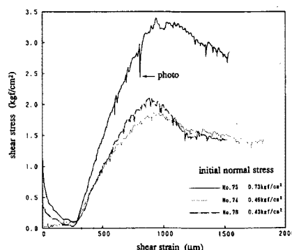
Fig. 8. Characteristics of shear strength (diluvial clay; V-section)
