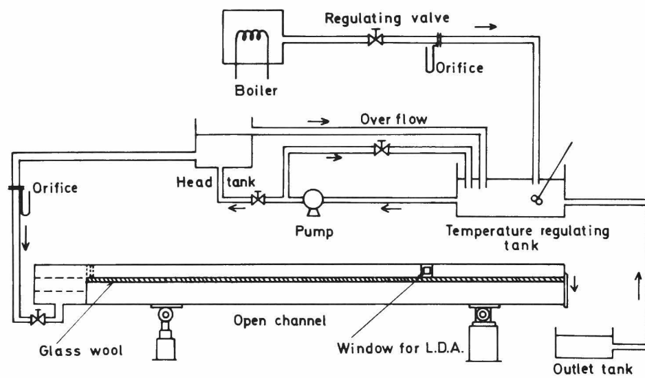
Figure 3.1. Flow system of experimental apparatus.
